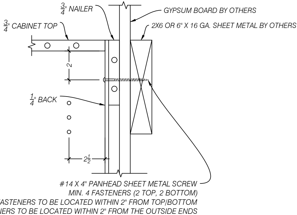
C ENLARGED DETAIL - BASE CABINET ATTACHMENT @ WALL SCALE 1:4 (3"=1'-0") ARCH REF: NA
