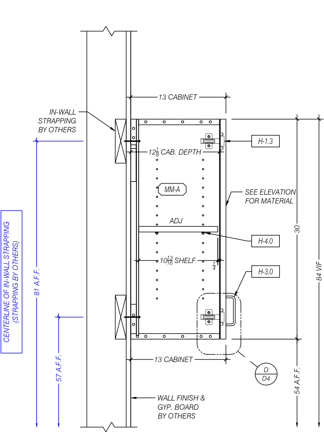
A SECTION - WALL CABINET SCALE 1:8 (1 1/2"=1'-0") ARCH REF: 13/AE581
