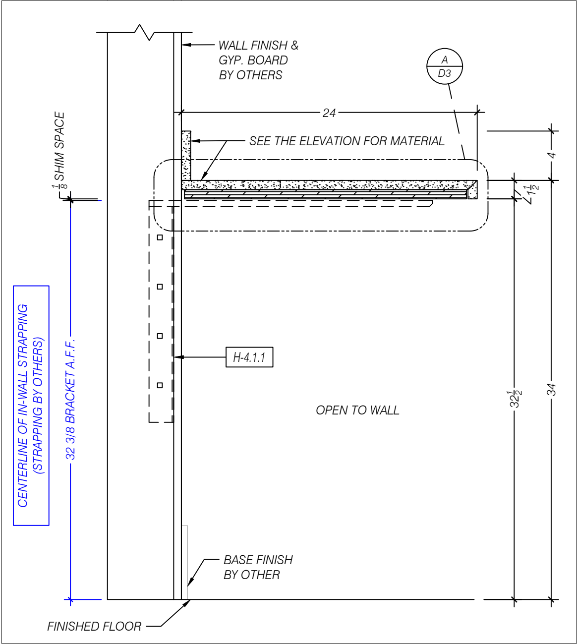
A SECTION - COUNTERTOP W/ BRACKET SCALE 1:8 (1 1/2"=1'-0") ARCH REF: 6/AE583
