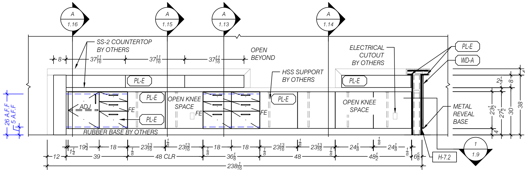
2 ELEVATION EAST - RECEPTION SCALE 1:24 (1/2"=1'-0") ARCH REF: 4/AE580
