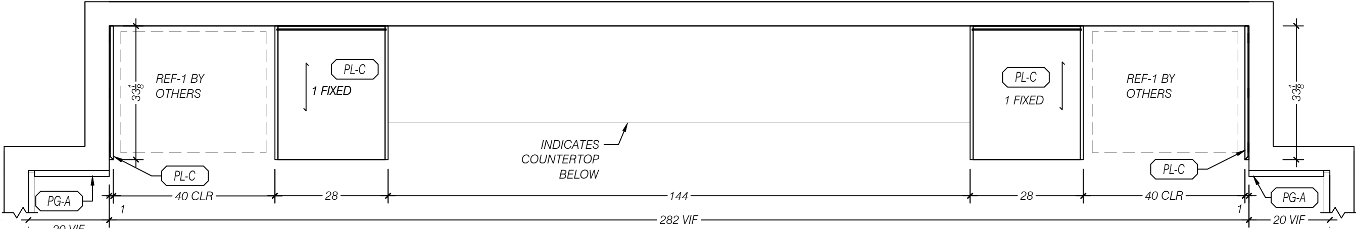
2 PLAN SECTION TALL - BREAK ROOM 115 SCALE 1:24 (1/2"=1'-0") ARCH REF: NA
