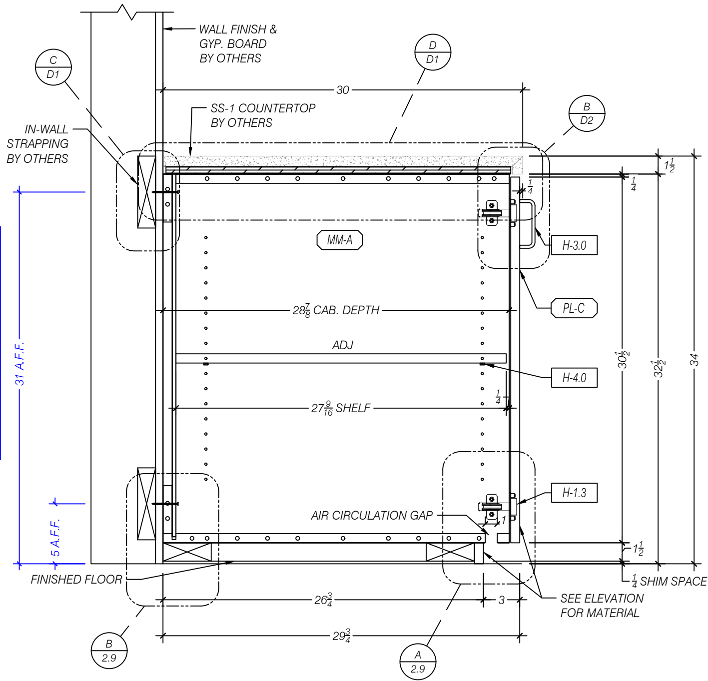
A SECTION - BASE CABINET SCALE 1:8 (1 1/2" = 1'-0") ARCH REF: 15/AE581
