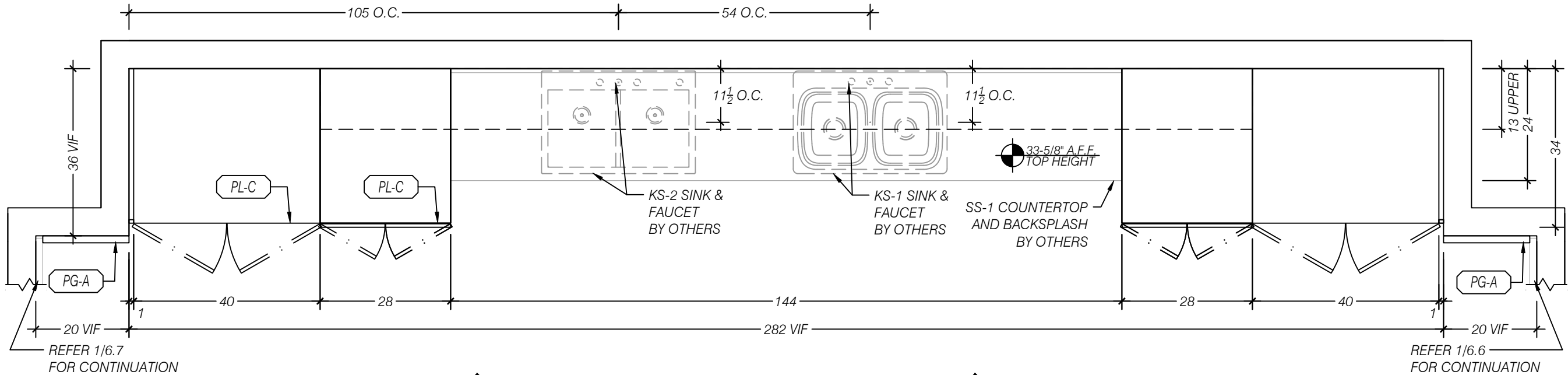
2 PLAN - BREAK ROOM 115 SCALE 1:24 (1/2"=1'-0") ARCH REF: 1/AE407
