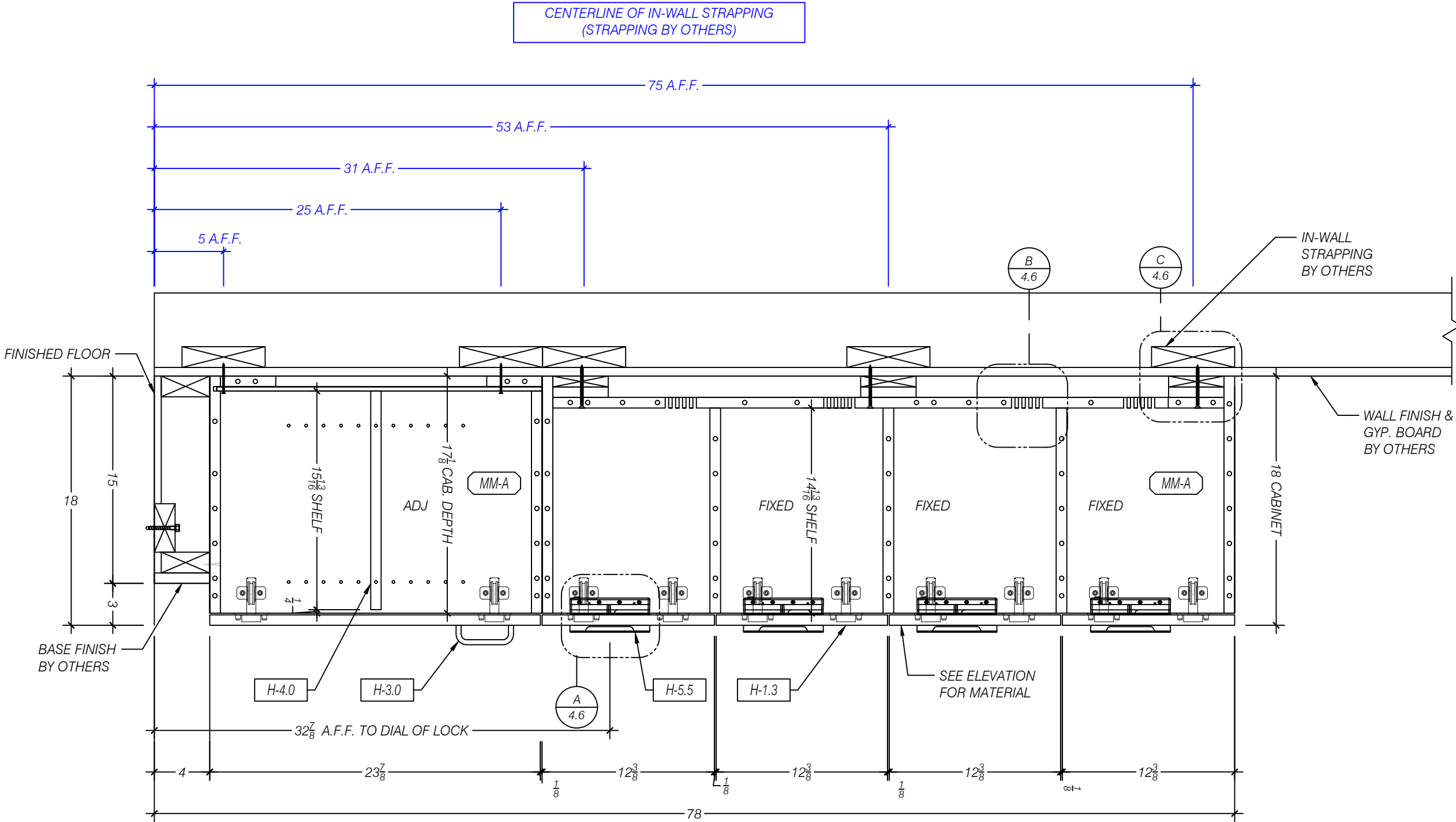
A SECTION - TALL CABINET SCALE 1:8 (1 1/2"=1'-0") ARCH REF: 22/AE582
