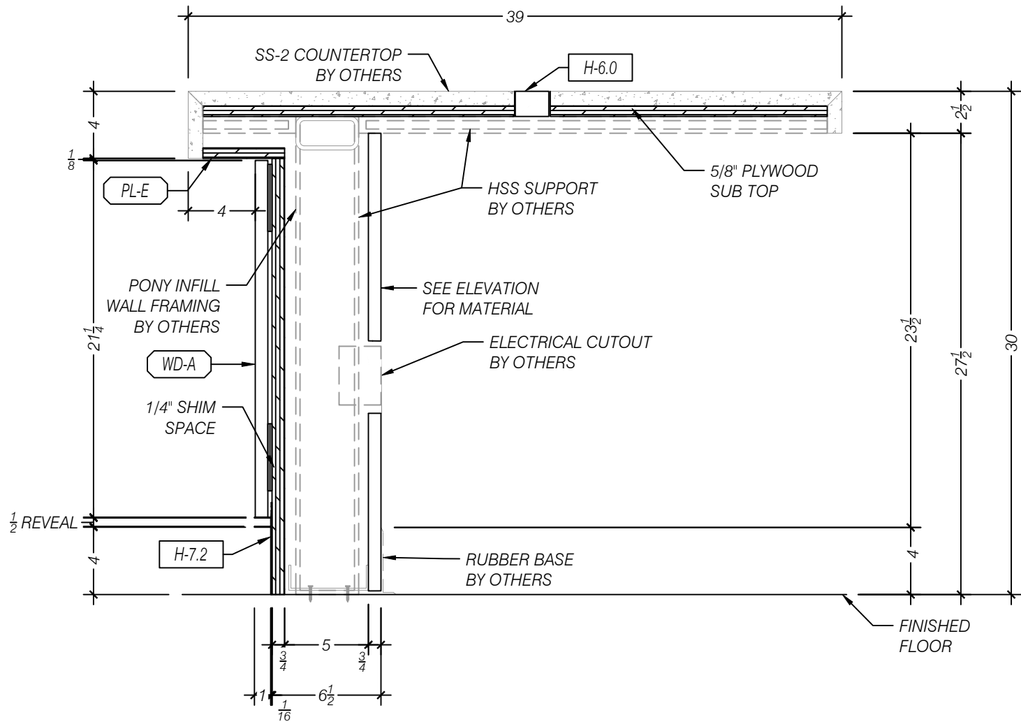
A SECTION - COUNTERTOP w/ TRANSACTION COUNTER SCALE 1:8 (1 1/2"=1'-0") ARCH REF: 2/AE584
