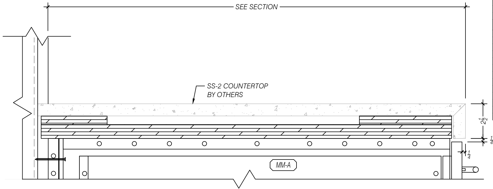
A ENLARGED DETAIL - COUNTERTOP DETAIL SCALE 1:4 (3"=1'-0") ARCH REF: NA
