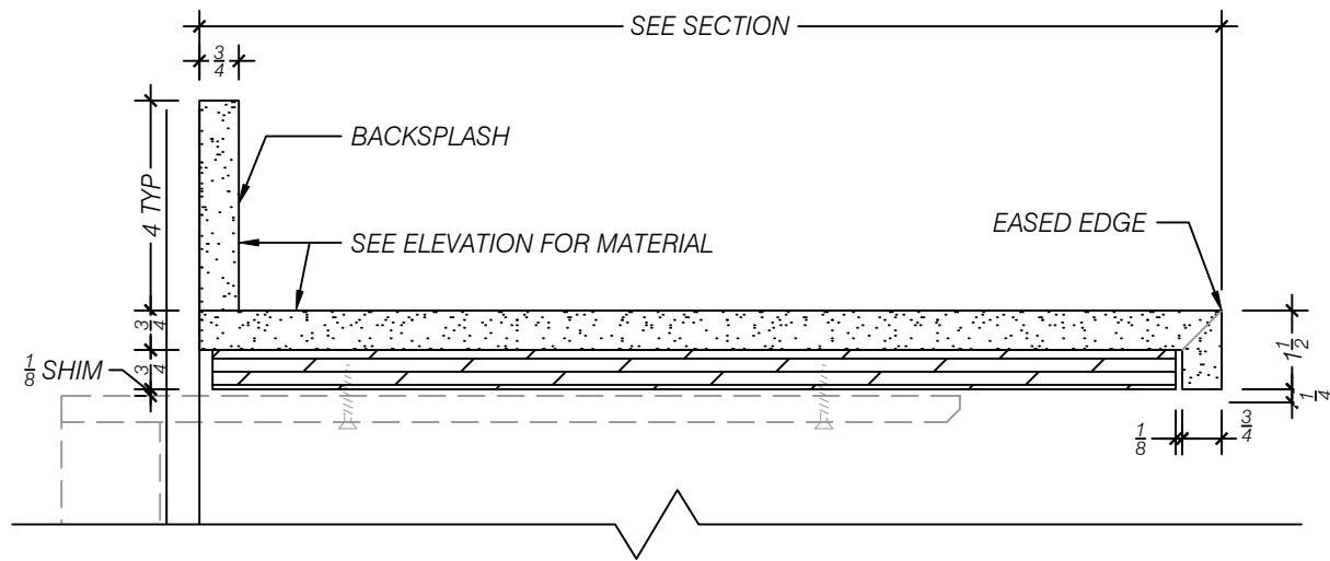
A ENLARGED DETAIL - P-LAM COUNTERTOP WITH BRACKETS SCALE 1:4 (3"=1'-0") ARCH REF: 11/AE584
