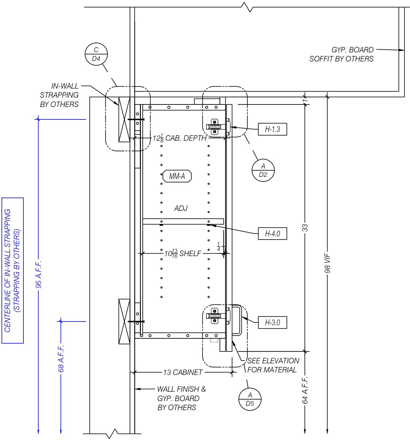
B SECTION - WALL CABINET w/ LIGHT VALANCE SCALE 1:8 (1 1/2"=1'-0") ARCH REF: 13/AE581
