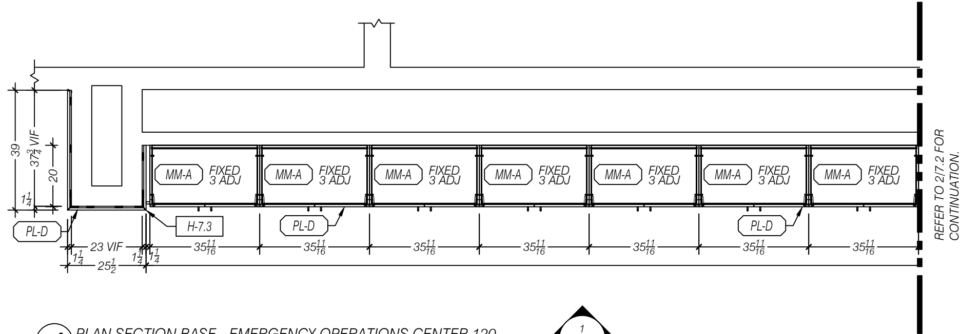
1 PLAN SECTION BASE - EMERGENCY OPERATIONS CENTER 120 SCALE 1:32 (3/8"=1'-0") ARCH REF: NA
