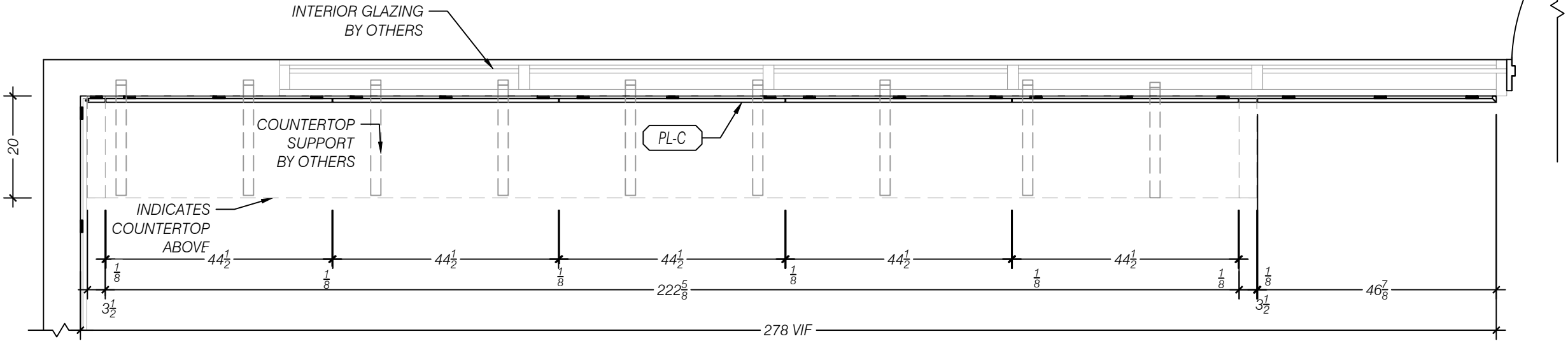
2 PLAN SECTION BASE - BREAK ROOM 115 SCALE 1:24 (1/2"=1'-0") ARCH REF: NA
