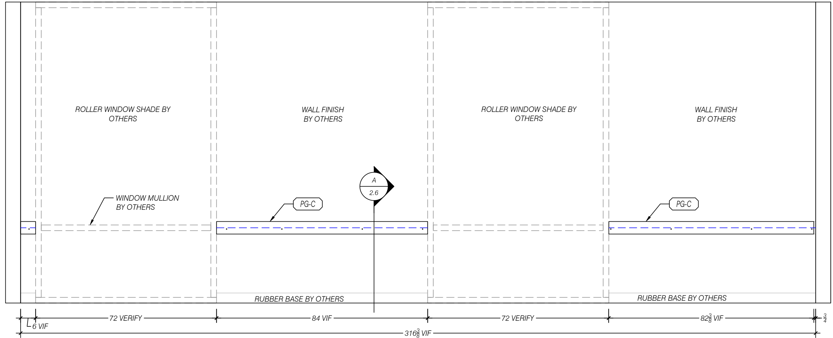
2 ELEVATION EAST - CONFERENCE 102 SCALE 1:24 (1/2"=1'-0") ARCH REF: 7/AE406
