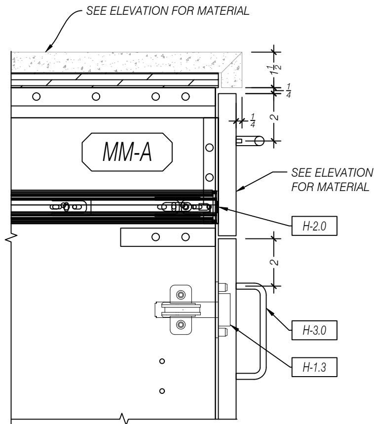
C ENLARGED DETAIL - DOOR/ DRAWER PULL LOCATION SCALE 1:4 (3"=1'-0") ARCH REF: NA
