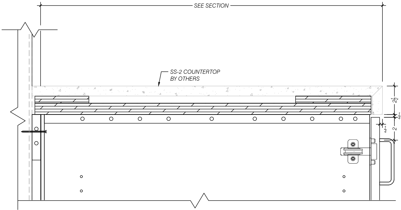
A ENLARGED DETAIL - DOOR PULL LOCATION SCALE 1:4 (3"=1'-0") ARCH REF: NA
