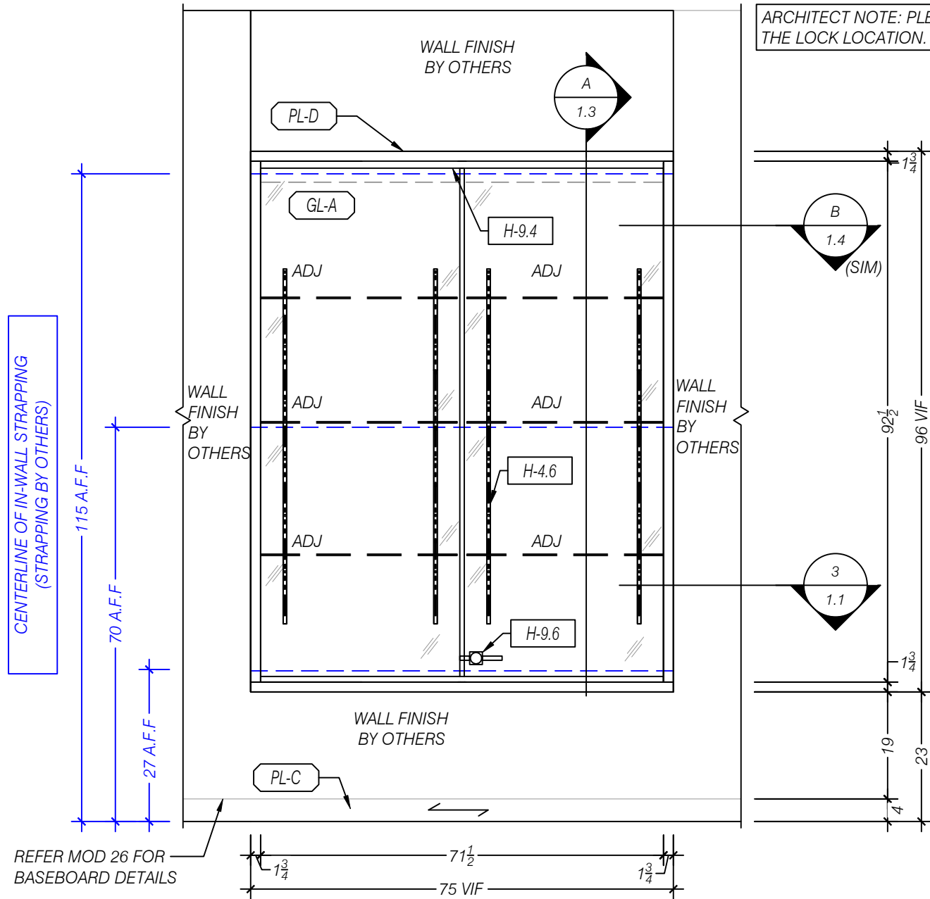
1 ELEVATION NORTH - LOBBY 100 SCALE 1:24 (1/2"=1'-0") ARCH REF: 3/AE401
