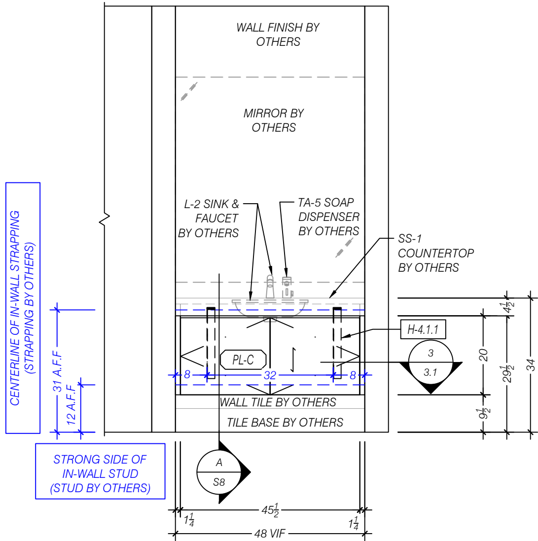
4 ELEVATION WEST - ALL GENDER 103 SCALE 1:24 (1/2"=1'-0") ARCH REF: 4/AE403
