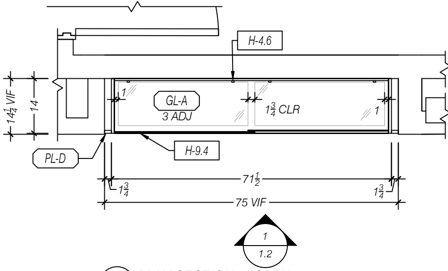
3 PLAN SECTION - LOBBY 100 SCALE 1:24 (1/2" = 1'-0") ARCH REF: 5/AE582
