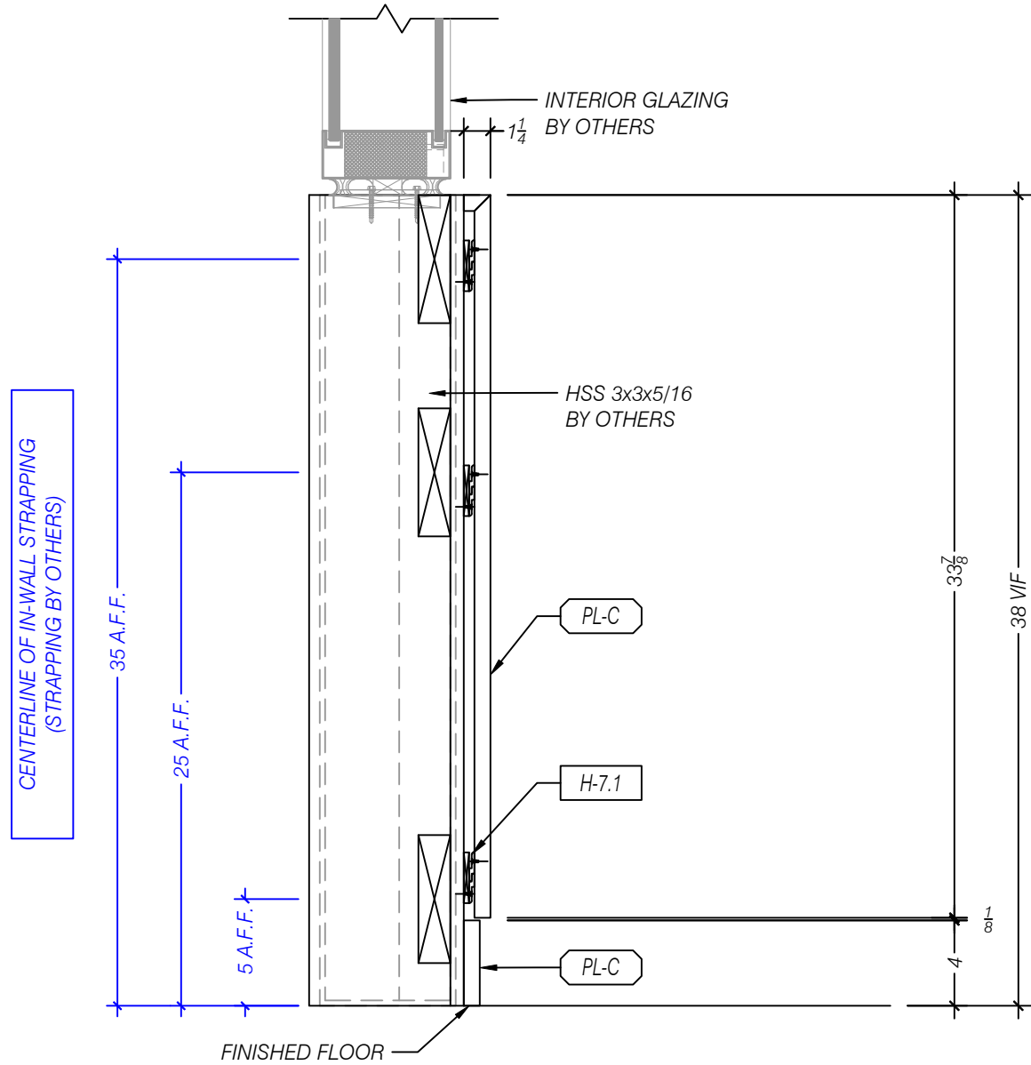
B SECTION - PANELING SCALE 1:8 (1 1/2"=1'-0") ARCH REF: NA
