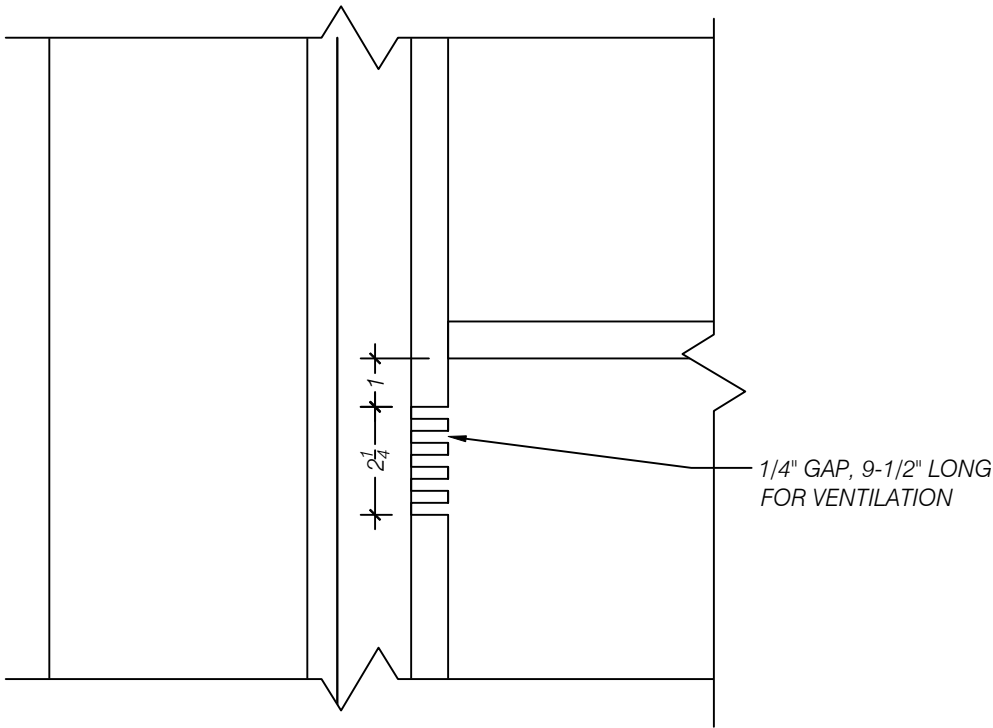
B ENLARGED DETAIL - LOCKER VENTILATION SCALE 1:4 (3"=1'-0") ARCH REF: NA
