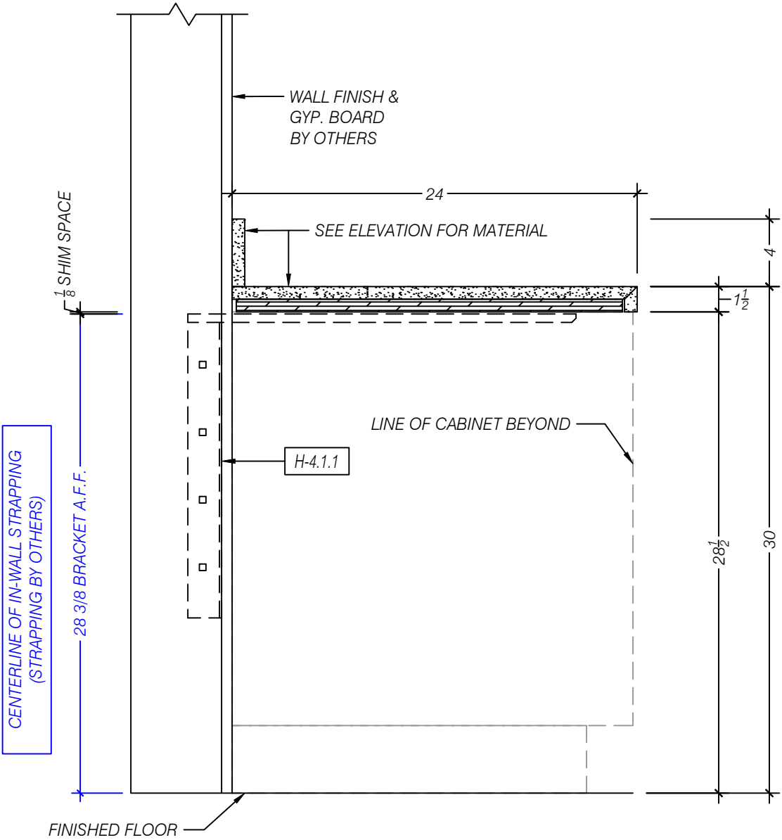
B SECTION - COUNTERTOP w/ BRACKET SCALE 1:8 (1 1/2"=1'-0") ARCH REF: 8/AE581
