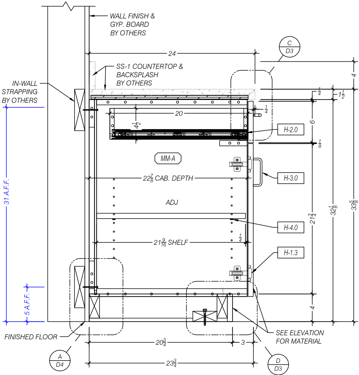
B SECTION - DOOR/DRAWER CABINET SCALE 1:8 (1 1/2"=1'-0") ARCH REF: 7/AE581
