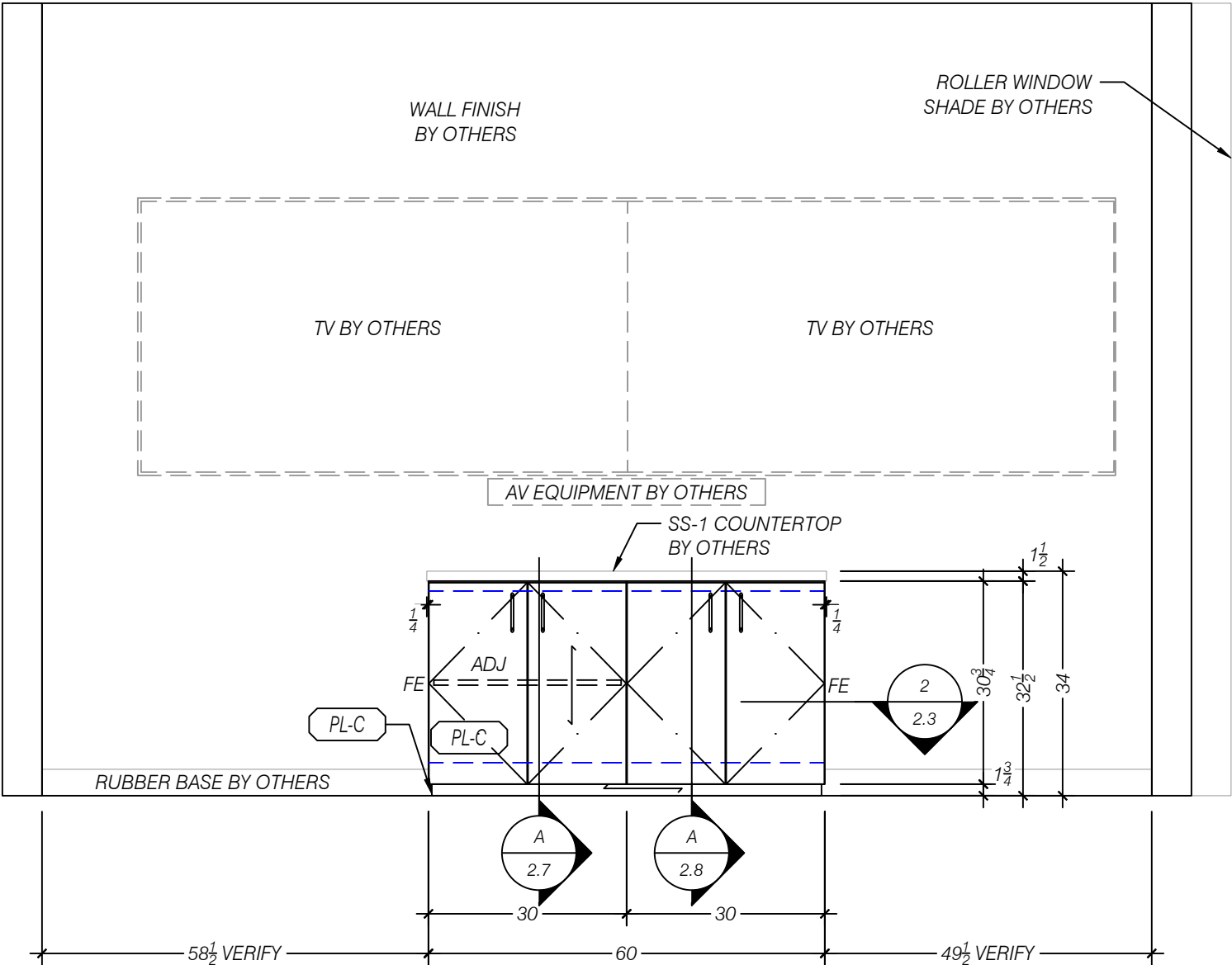
1 ELEVATION NORTH - CONFERENCE 102 SCALE 1:24 (1/2" = 1'-0") ARCH REF: 6/AE406
