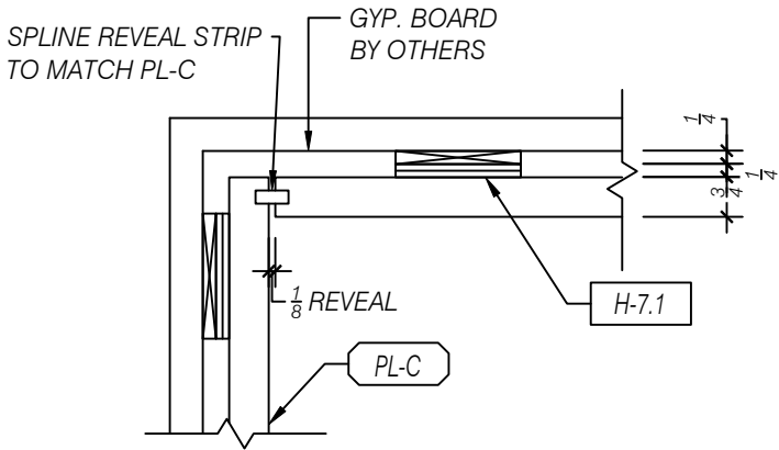
B ENLARGED DETAIL - PANEL TO PANEL REVEAL SCALE 1:4 (3"=1'-0") NA
