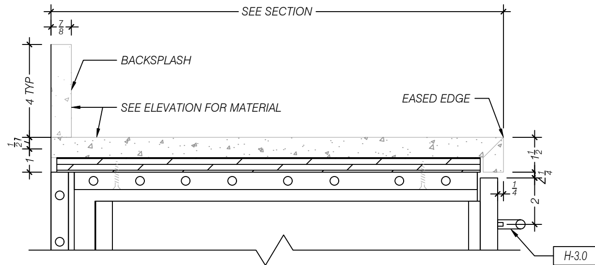
B ENLARGED DETAIL - COUNTERTOP DETAIL SCALE 1:4 (3"=1'-0") ARCH REF: 11/AE584
