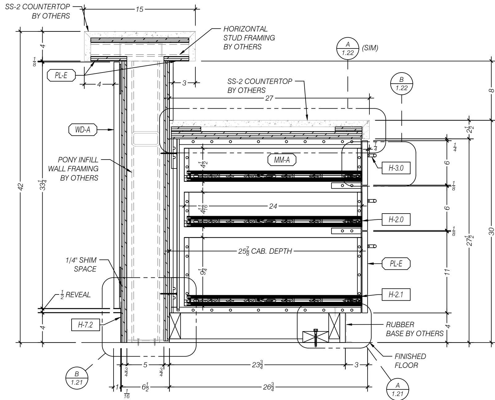
A SECTION - 3 DRAWER BASE CABINET w/ TRANSACTION COUNTER SCALE 1:8 (1 1/2"=1'-0") ARCH REF: 1/AE584
