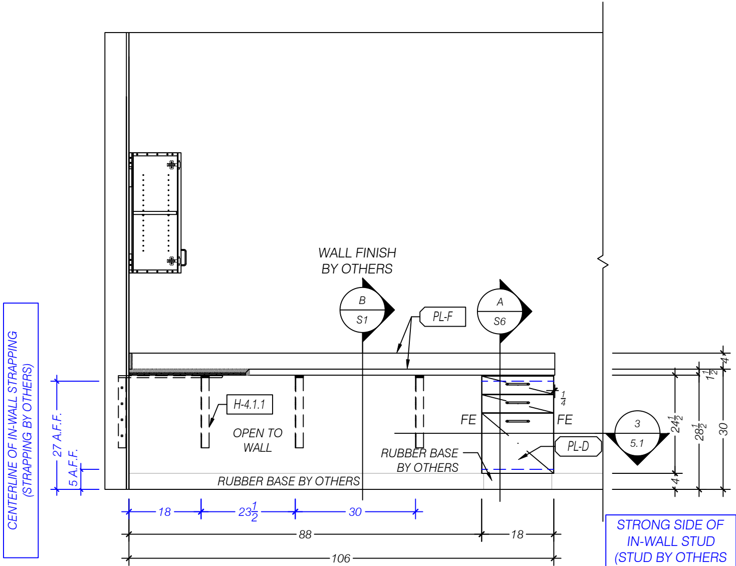
2 ELEVATION SOUTH - MEDIA CONTROL 113 SCALE 1:24 (1/2"=1'-0") ARCH REF: 8/AE408
