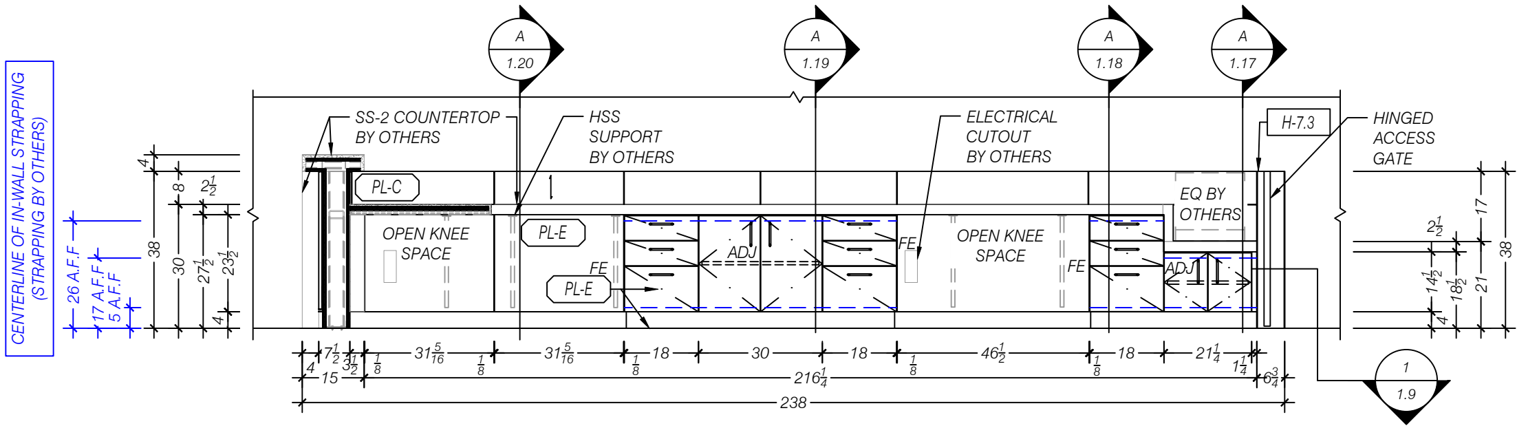
2 ELEVATION WEST- RECEPTION SCALE 1:24 (1/2"=1'-0") ARCH REF: 2/AE580
