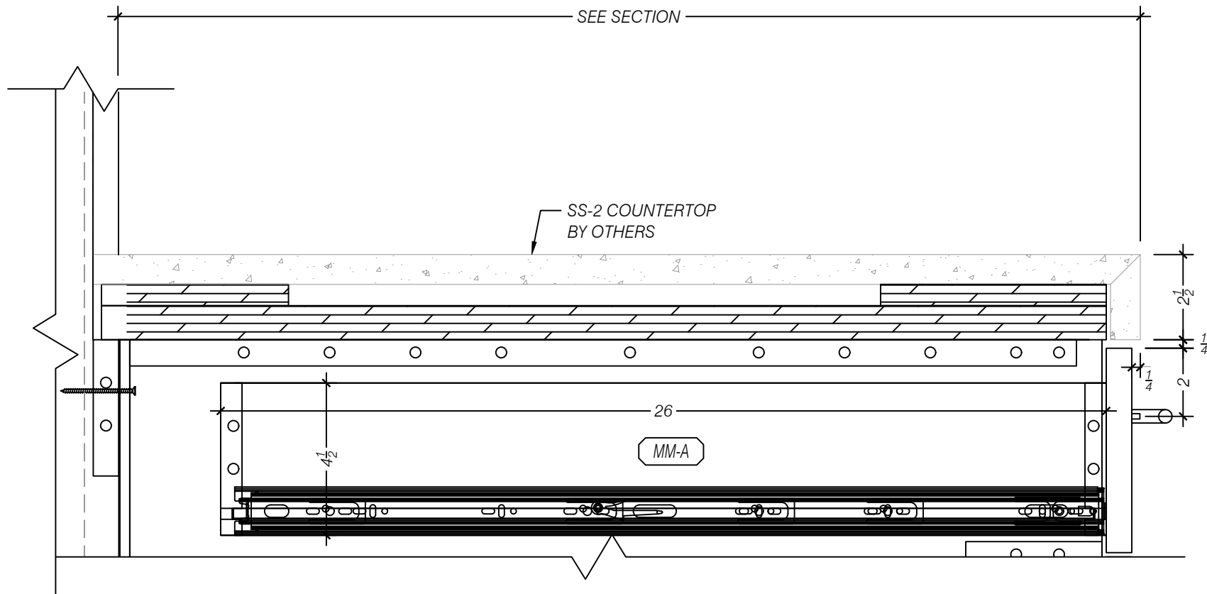
B ENLARGED DETAIL - DRAWER PULL LOCATION SCALE 1:4 (3"=1'-0") ARCH REF: NA
