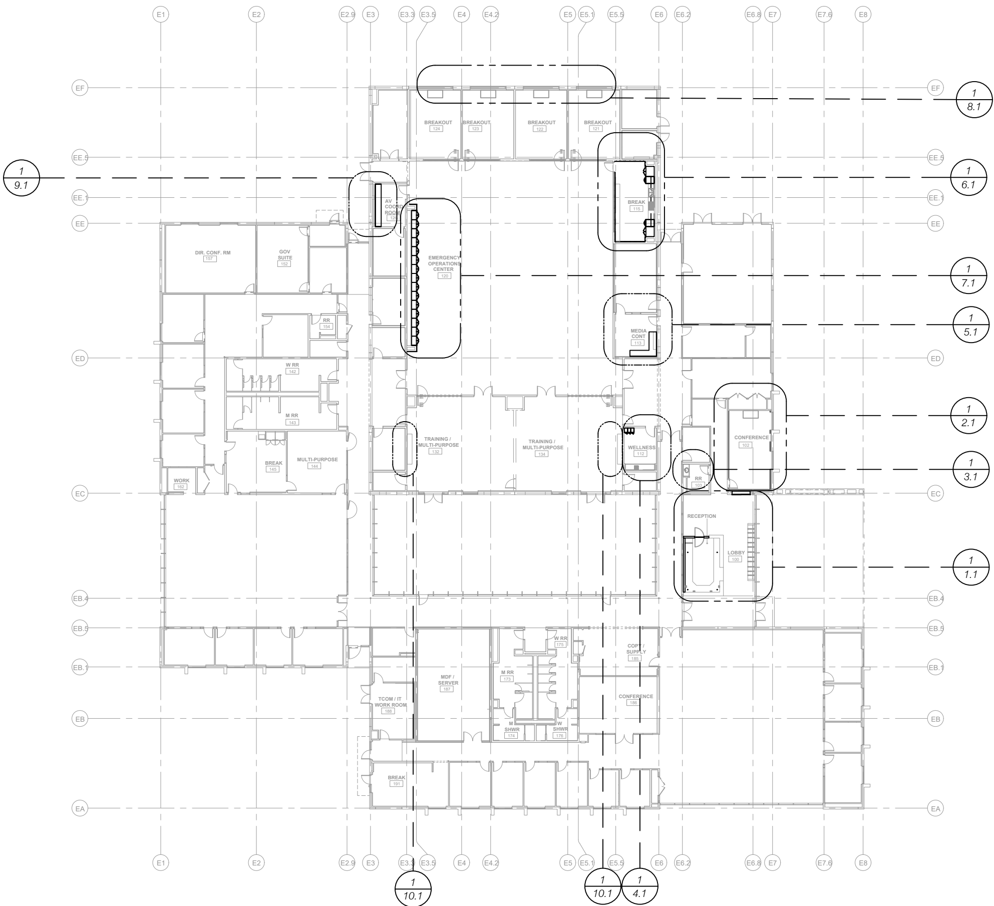
1 OVERALL FLOOR PLAN - LEVEL - 1 SCALE: NTS ARCH REF: 1/ AE101
