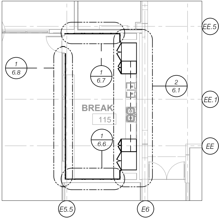
1 KEY PLAN SCALE: NTS ARCH REF: 1/AE101.1
