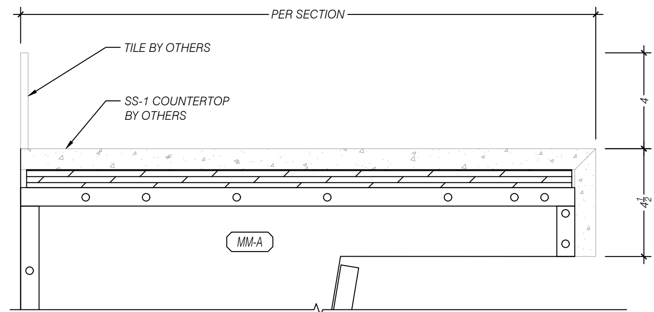
D ENLARGED DETAIL - COUNTERTOP DETAIL SCALE 1:4 (3"=1'-0") ARCH REF: NA
