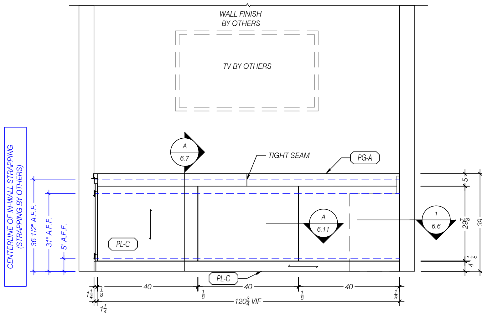
2 ELEVATION SOUTH - BREAK ROOM 115 SCALE 1:24 (1/2"=1'-0") ARCH REF: 4/AE407
