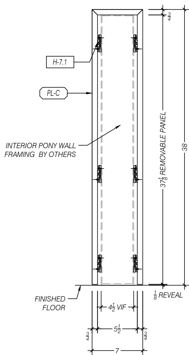
C SECTION - PANEL PARTITION SCALE 1:8 (1 1/2" = 1'-0") ARCH REF: NA
