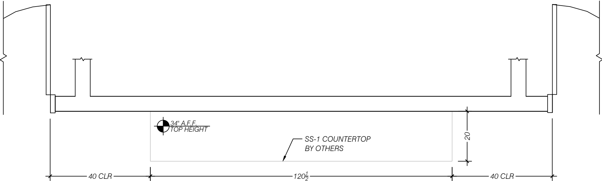
2 PLAN - TRAINING/MULTI-PURPOSE ROOM 134 SCALE 1:24 (1/2"=1'-0") ARCH REF: 1/AE415
