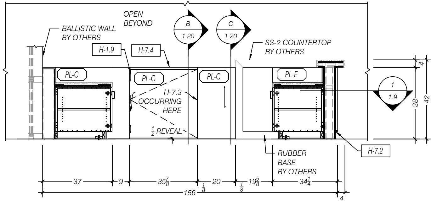
1 ELEVATION NORTH - RECEPTION SCALE 1:24 (1/2"=1'-0") ARCH REF: 3/AE580
