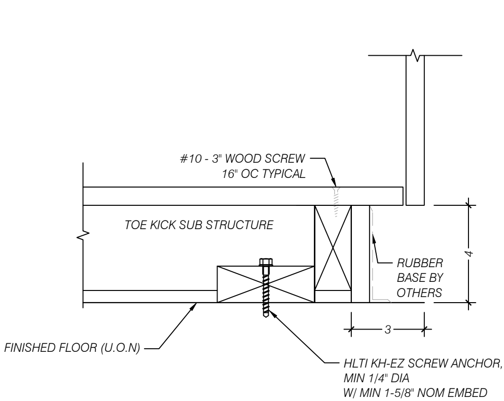
A ENLARGED DETAIL - TOE KICK FACE SCALE 1:4 (3"=1'-0") ARCH REF: NA
