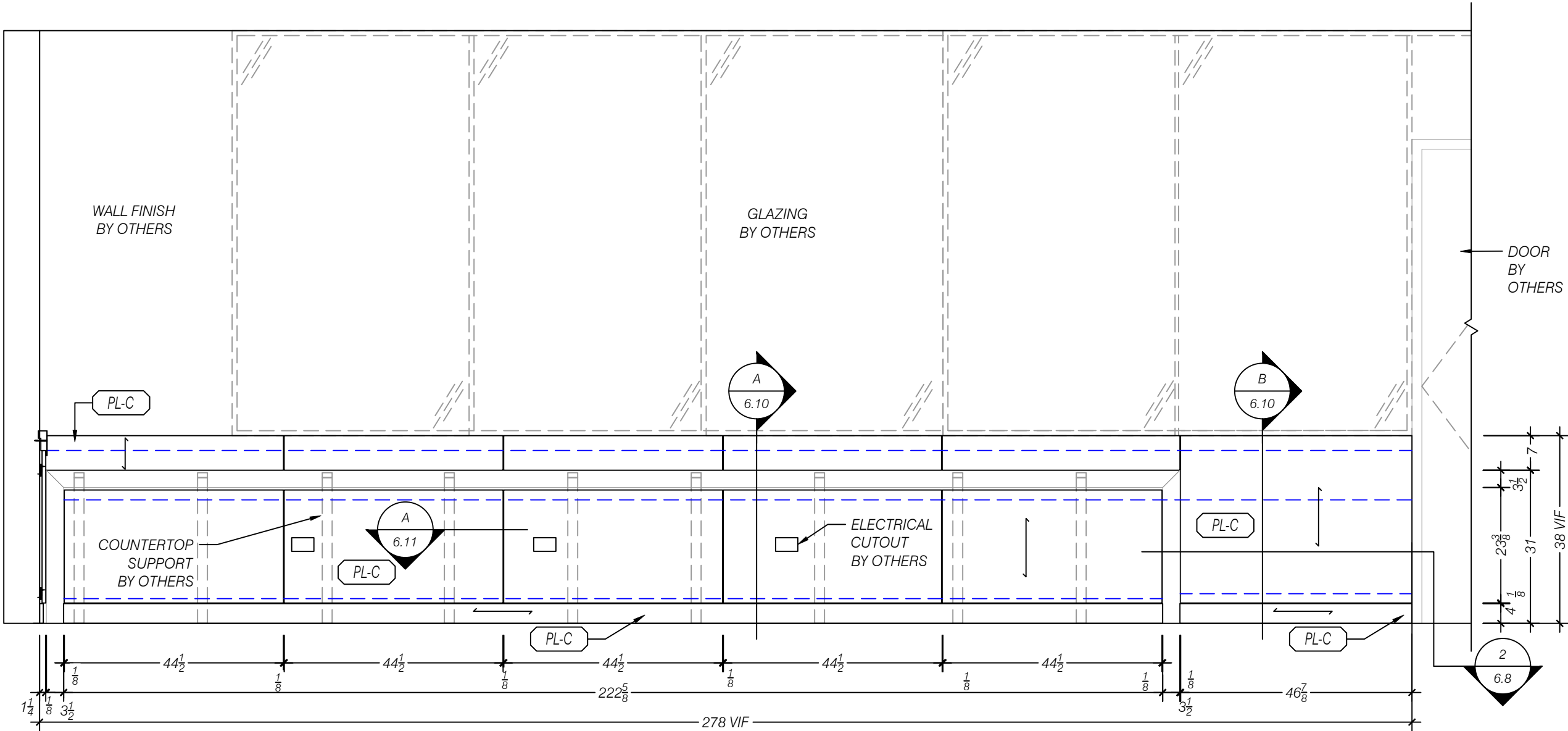
1 ELEVATION WEST - BREAK ROOM 115 SCALE 1:24 (1/2"=1'-0") ARCH REF: 5/AE407
