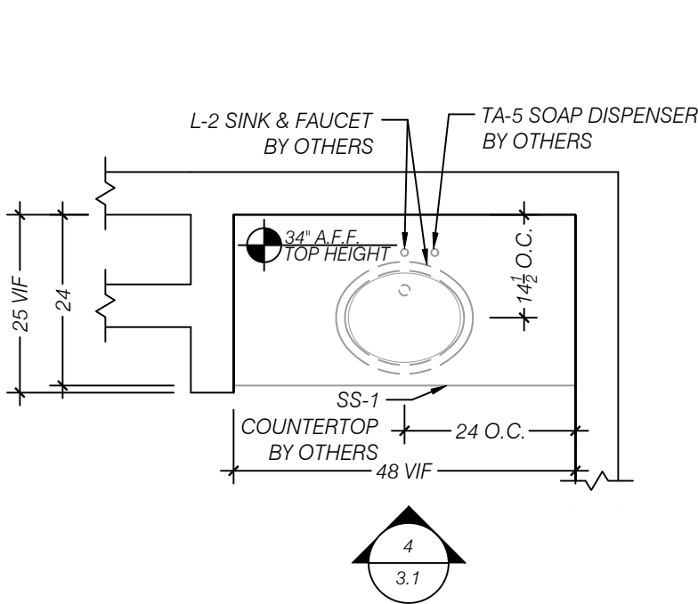
2 PLAN - ALL GENDER 103 SCALE 1:24 (1/2"=1'-0") ARCH REF: 4/AE402
