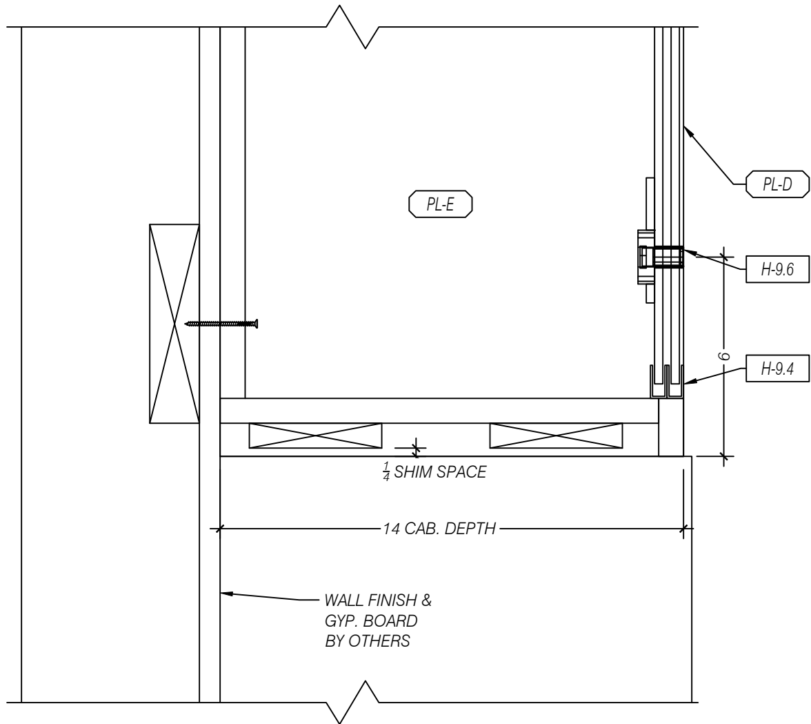
B ENLARGED DETAIL - SLIDING DOOR w/ TRIM SCALE 1:4 (3"=1'-0") ARCH REF: NA
