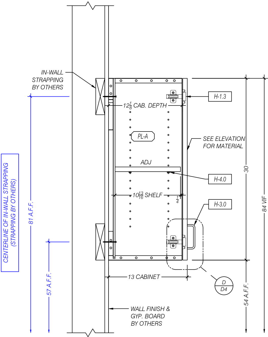
A SECTION - WALL CABINET SCALE 1:8 (1 1/2"=1'-0") ARCH REF: 13/AE581
