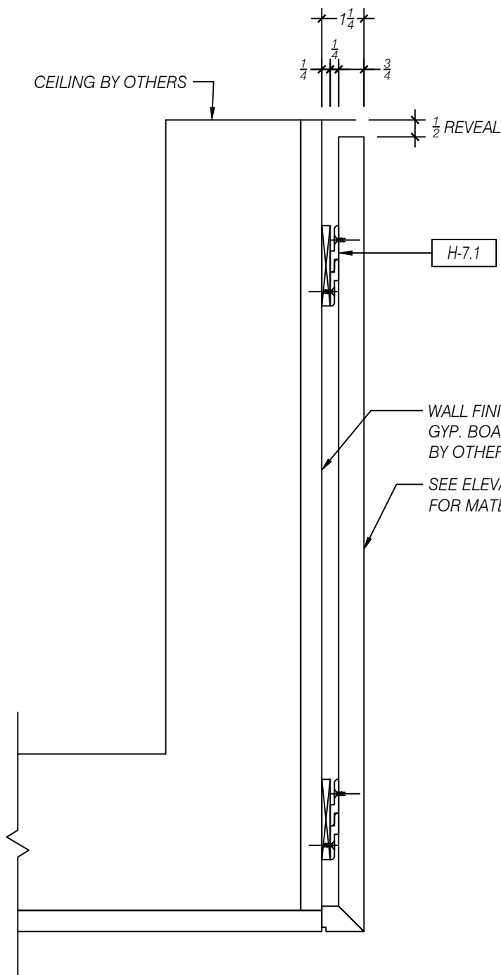
A ENLARGED DETAIL - WALL PANELING SCALE 1:4 (3"=1'-0") ARCH REF: NA
