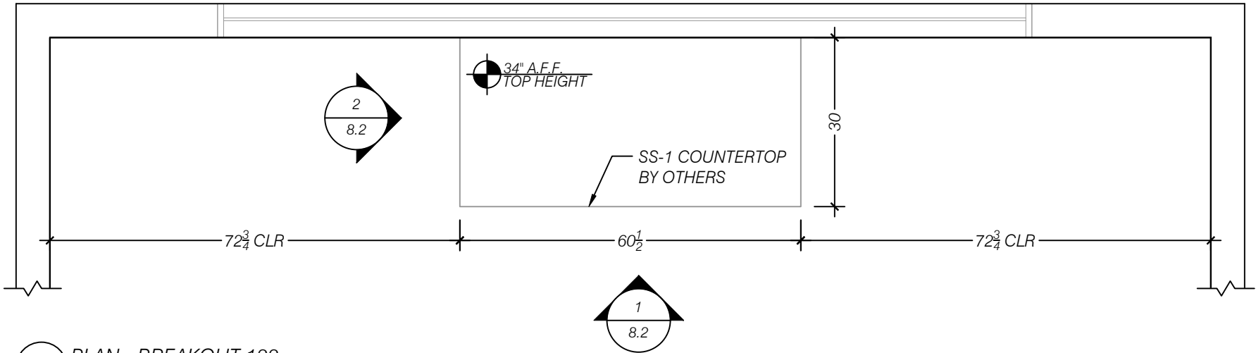
2 PLAN - BREAKOUT 122 SCALE 1:12 (1"=1'-0") ARCH REF: 6/AE407
