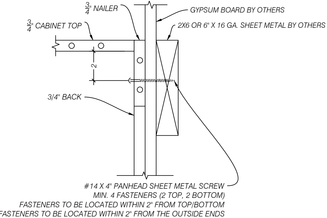
D ENLARGED DETAIL - THICK BACK CABINET ATTACHEMENT @ WALL SCALE 1:4 (3"=1'-0") ARCH REF: NA
