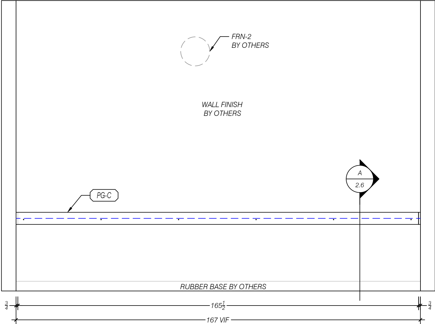
2 ELEVATION SOUTH - CONFERENCE 102 SCALE 1:24 (1/2"=1'-0") ARCH REF: 8/AE406
