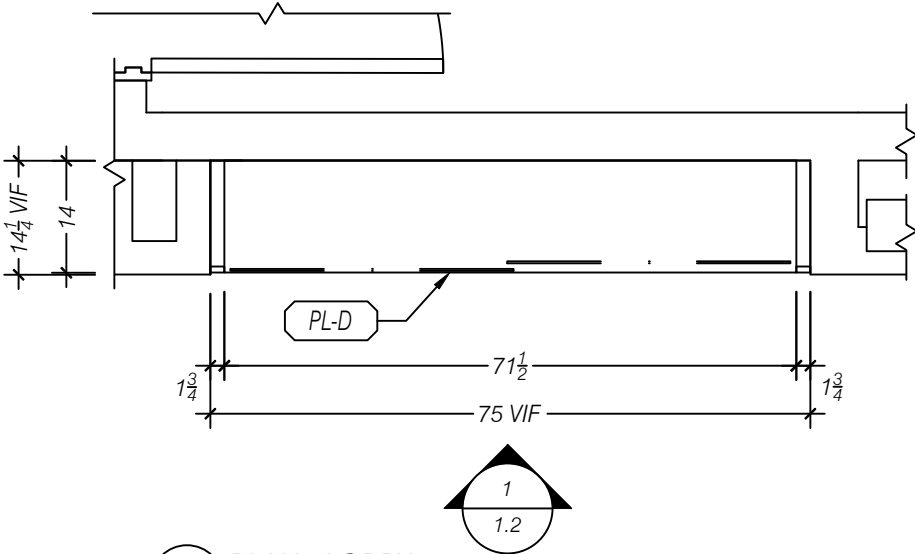
2 PLAN - LOBBY 100 SCALE 1:24 (1/2" = 1'-0") ARCH REF: 1/AE401
