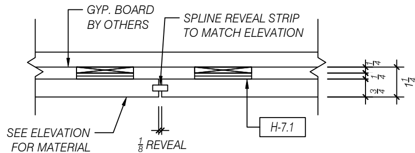
D ENLARGED DETAIL - PANEL TO PANEL REVEAL SCALE 1:4 (3"=1'-0") ARCH REF: NA
