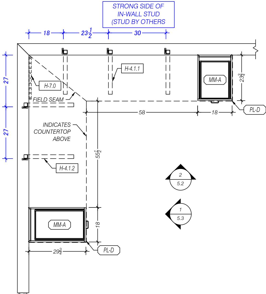
3 PLAN SECTION BASE - MEDIA CONTROL 113 SCALE 1:24 (1/2"=1'-0") ARCH REF: NA
