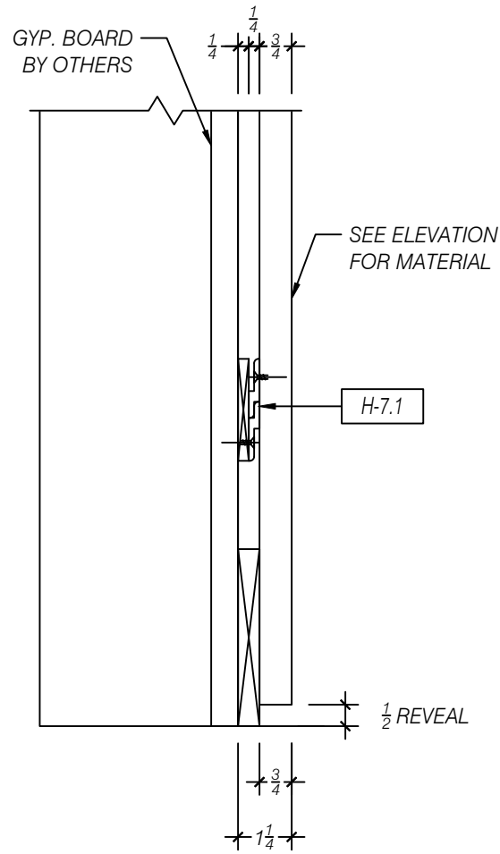
B ENLARGED DETAIL - PANEL TO BASE SCALE 1:4 (3"=1'-0") ARCH REF: NA
