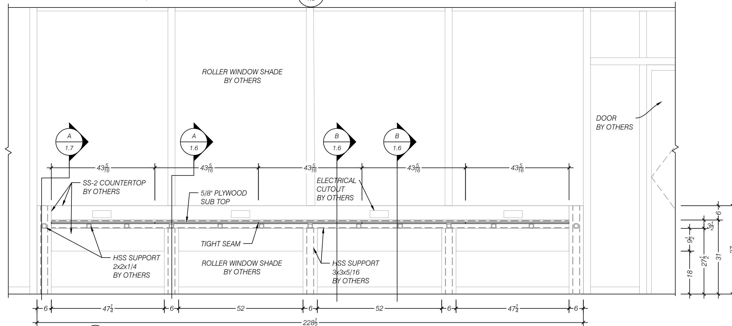
2 ELEVATION EAST - LOBBY 100 SCALE 1:24 (1/2"=1'-0") ARCH REF: 6/AE401
