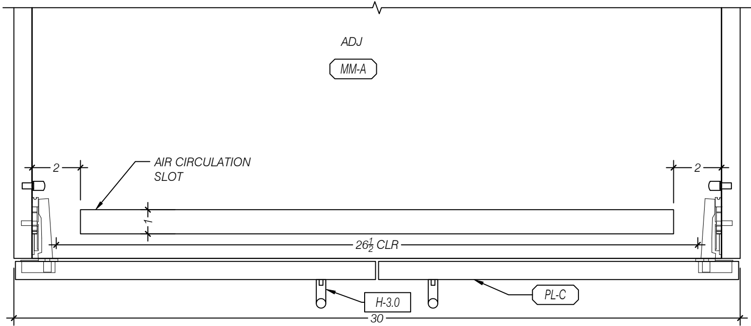
A ENLARGED DETAIL - AIR VENTILATION DETAIL SCALE 1:4 (3"=1'-0") ARCH REF: NA
