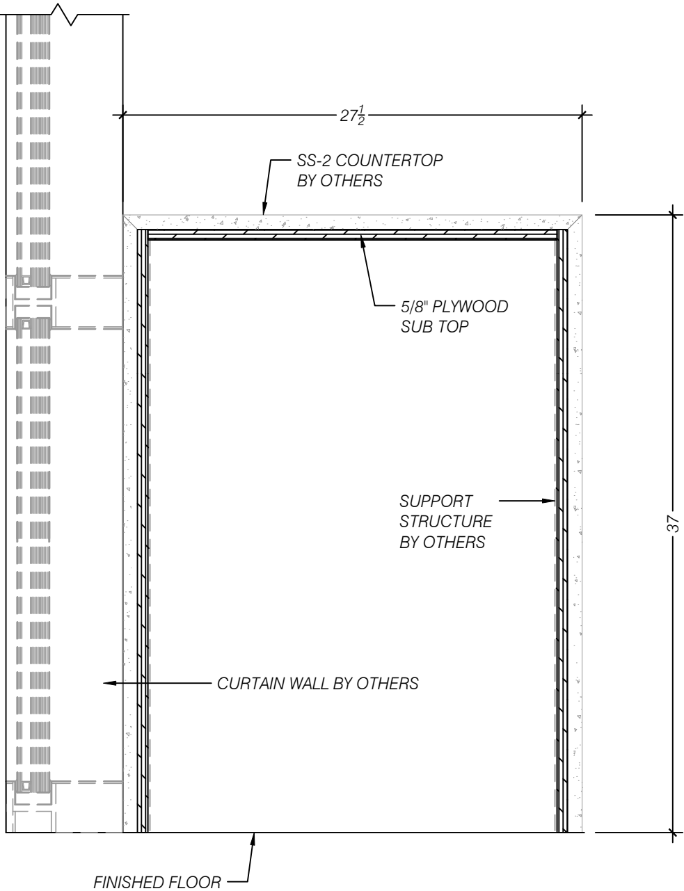
A SECTION - COUNTERTOP @ MULLION SCALE 1:8 (1 1/2"=1'-0") ARCH REF: NA
