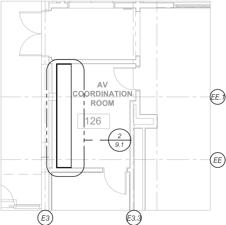
1 KEY PLAN SCALE : NTS ARCH REF: 1/AE101.1
