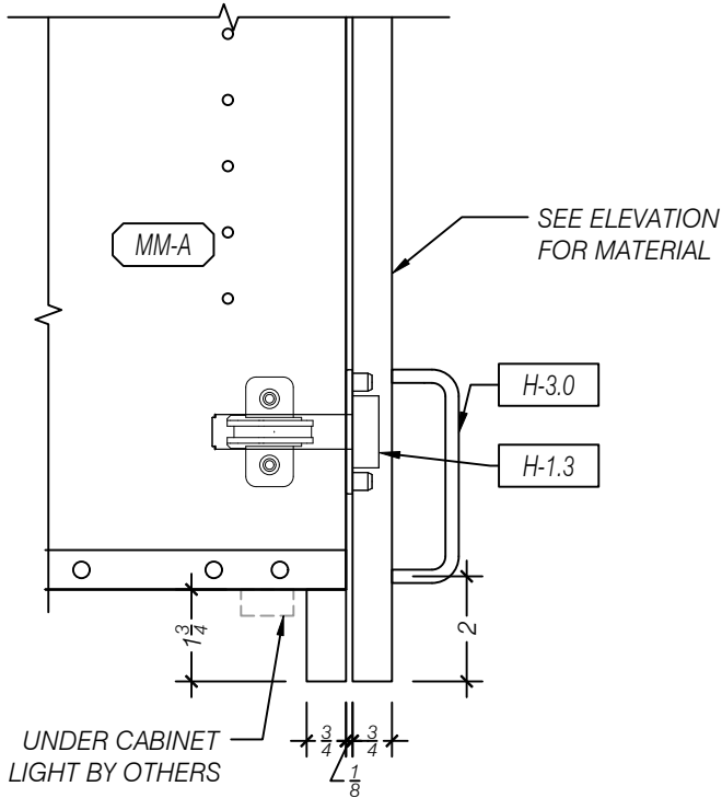
A ENLARGED DETAIL - UPPER CABINET PULL LOCATION w/ LIGHT VALANCE SCALE 1:4 (3"=1'-0") ARCH REF: NA
