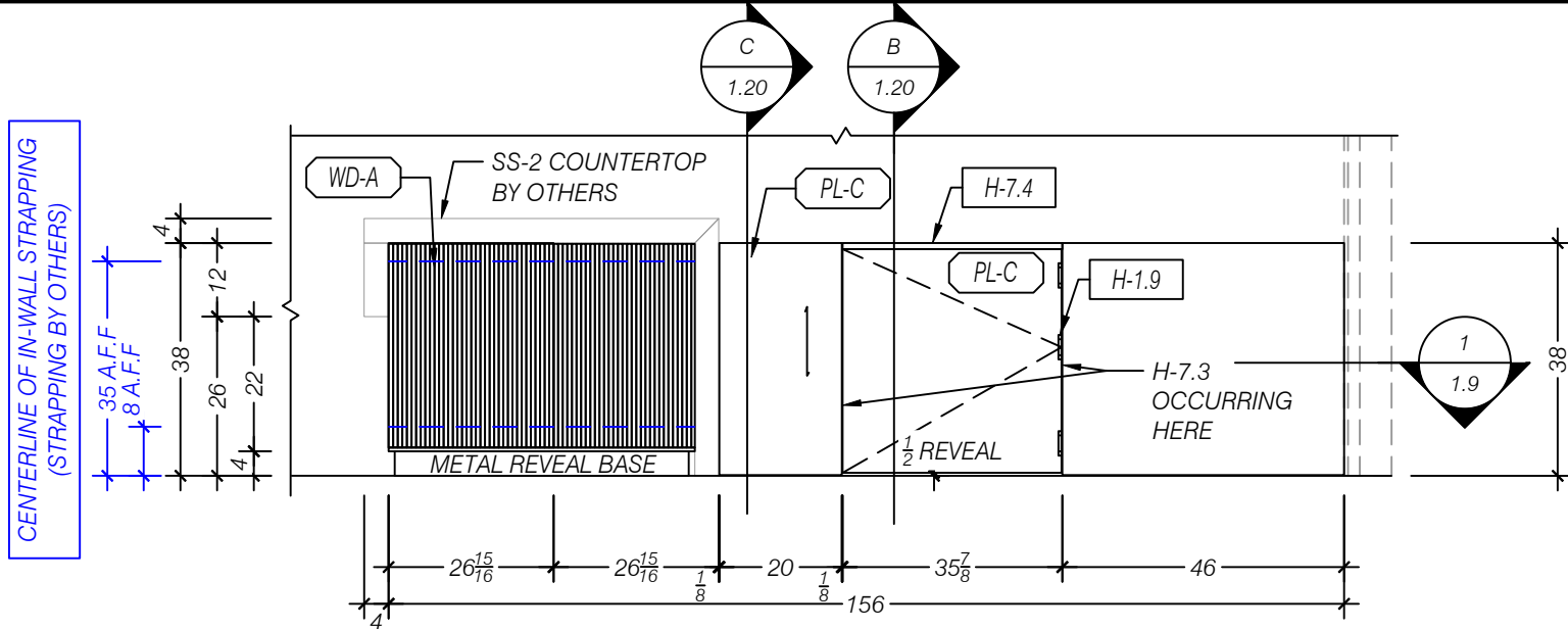
1 ELEVATION NORTH - RECEPTION SCALE 1:24 (1/2"=1'-0") ARCH REF: 8/AE580
