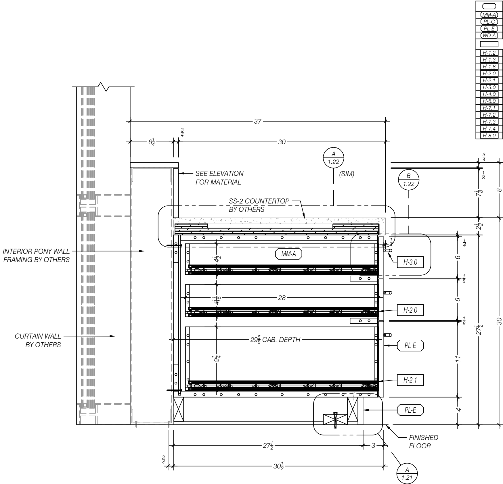
A SECTION - 3 DRAWER BASE CABINET w/ TRANSACTION COUNTER SCALE 1:8 (1 1/2"=1'-0") ARCH REF: 6/AE584
