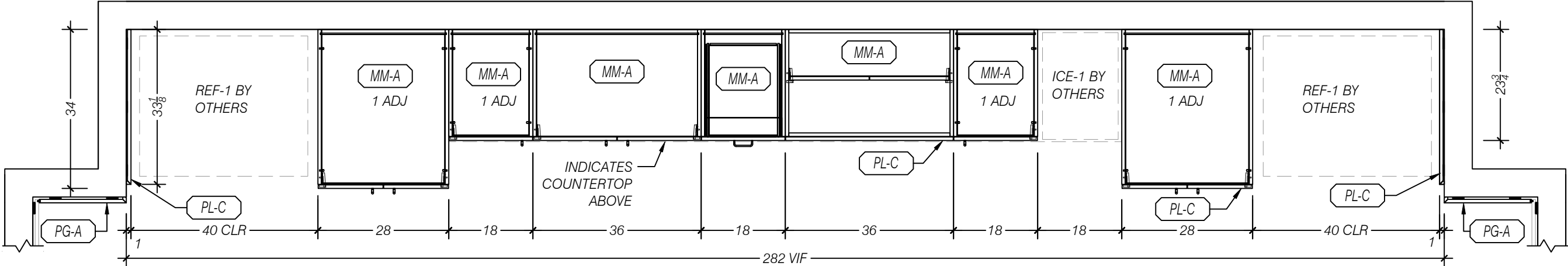
1 PLAN SECTION BASE - BREAK ROOM 115 SCALE 1:24 (1/2"=1'-0") ARCH REF: NA
