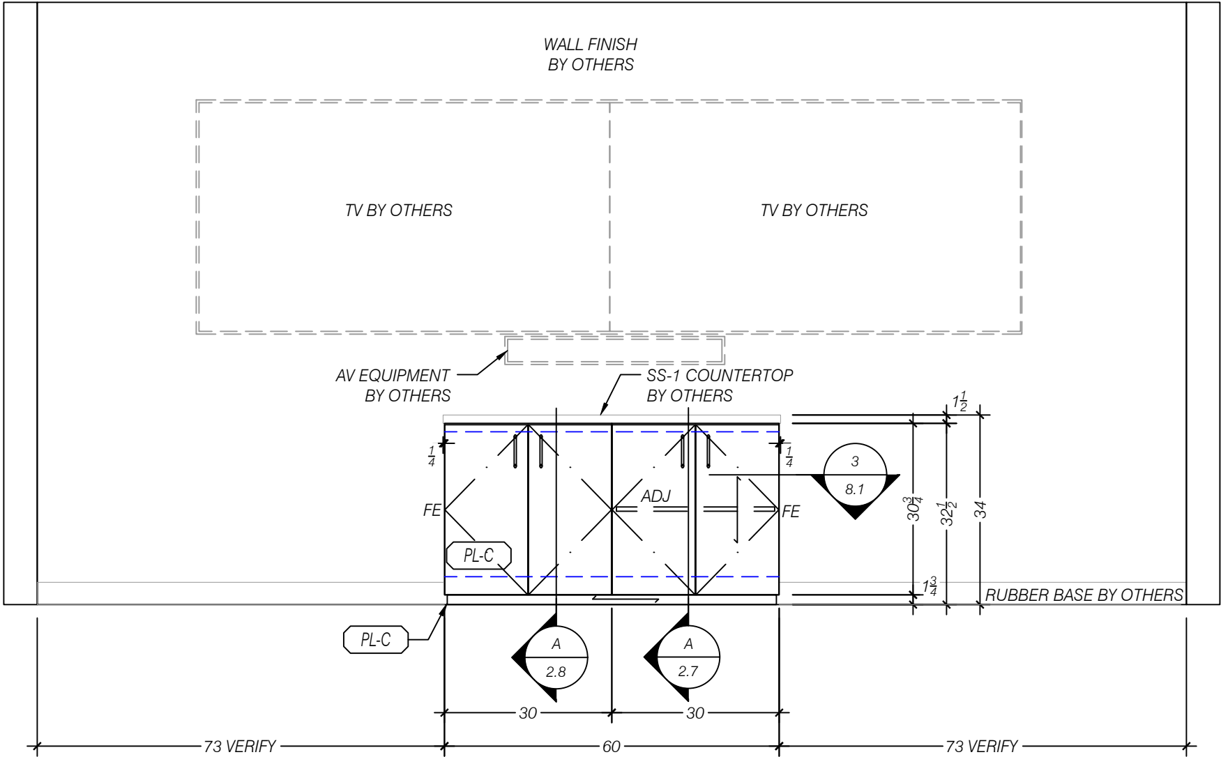
1 ELEVATION NORTH - BREAKOUT 122 SCALE 1:12 (1"=1'-0") ARCH REF: 7/AE407
