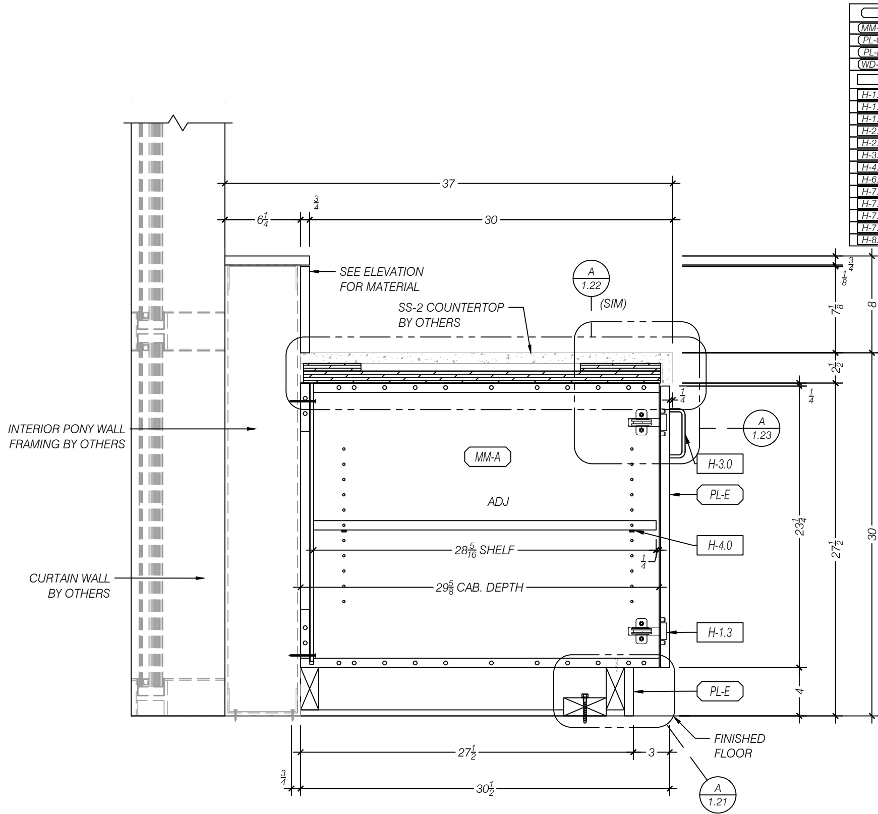
A SECTION - BASE CABINET w/ DOOR SCALE 1:8 (1 1/2"=1'-0") ARCH REF: 7/AE584
