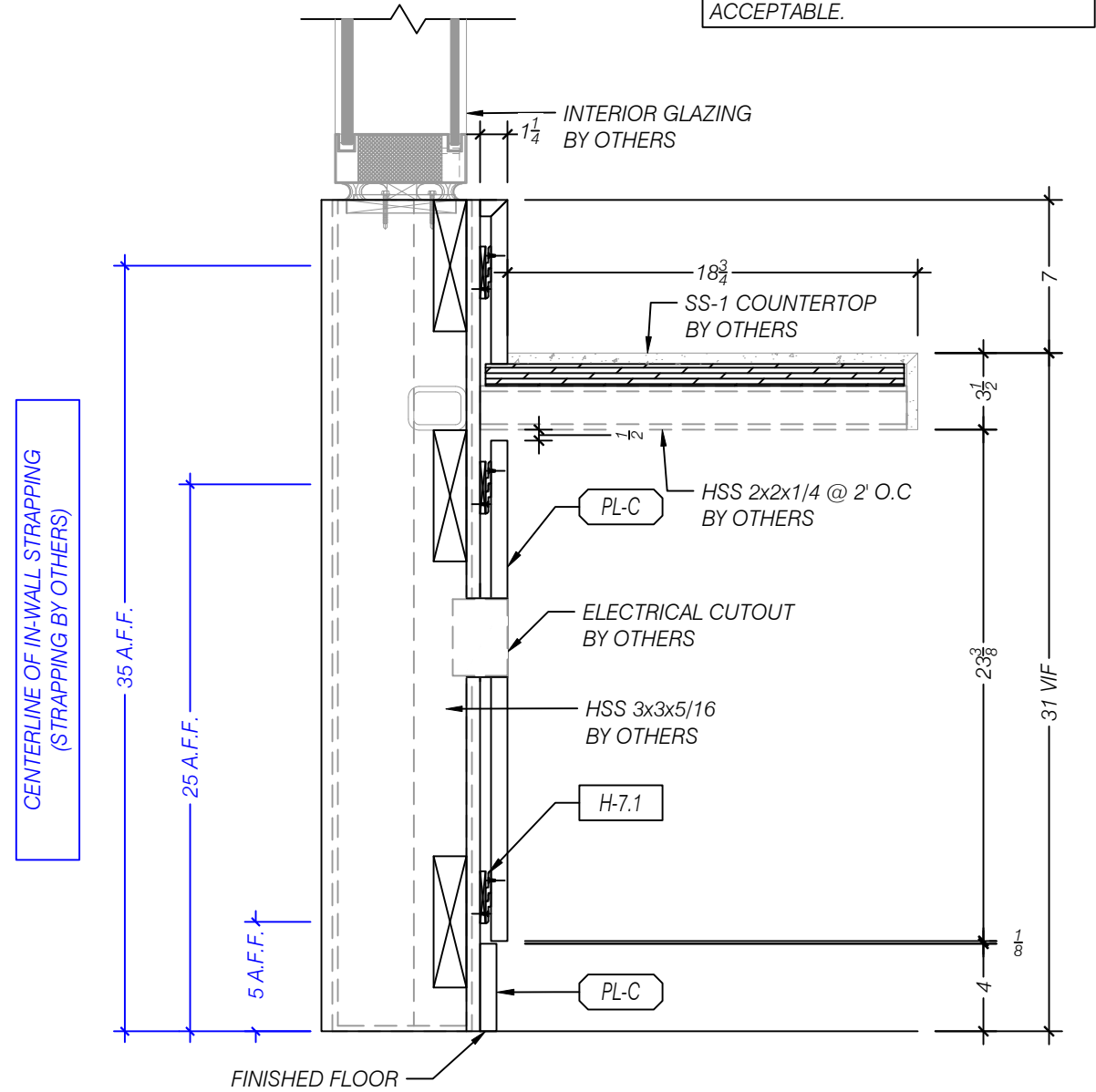
A SECTION - COUNTERTOP WITH PANELING SCALE 1:8 (1 1/2"=1'-0") ARCH REF: 5/AE583
