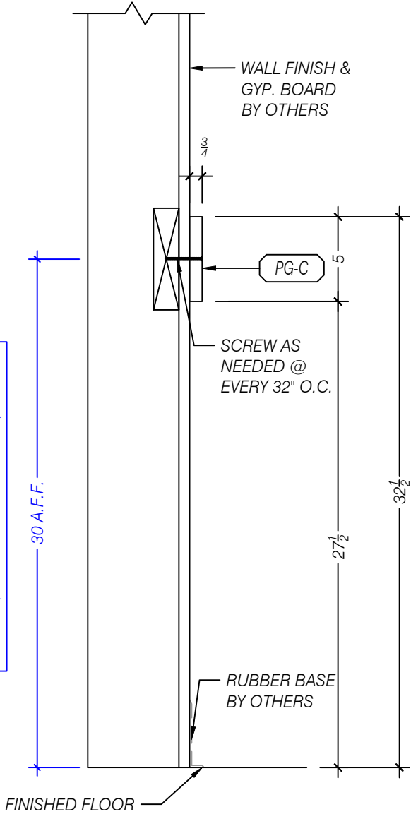
A SECTION - CHAIR RAIL SCALE 1:8 (1 1/2"=1'-0") ARCH REF: 3/AE585
