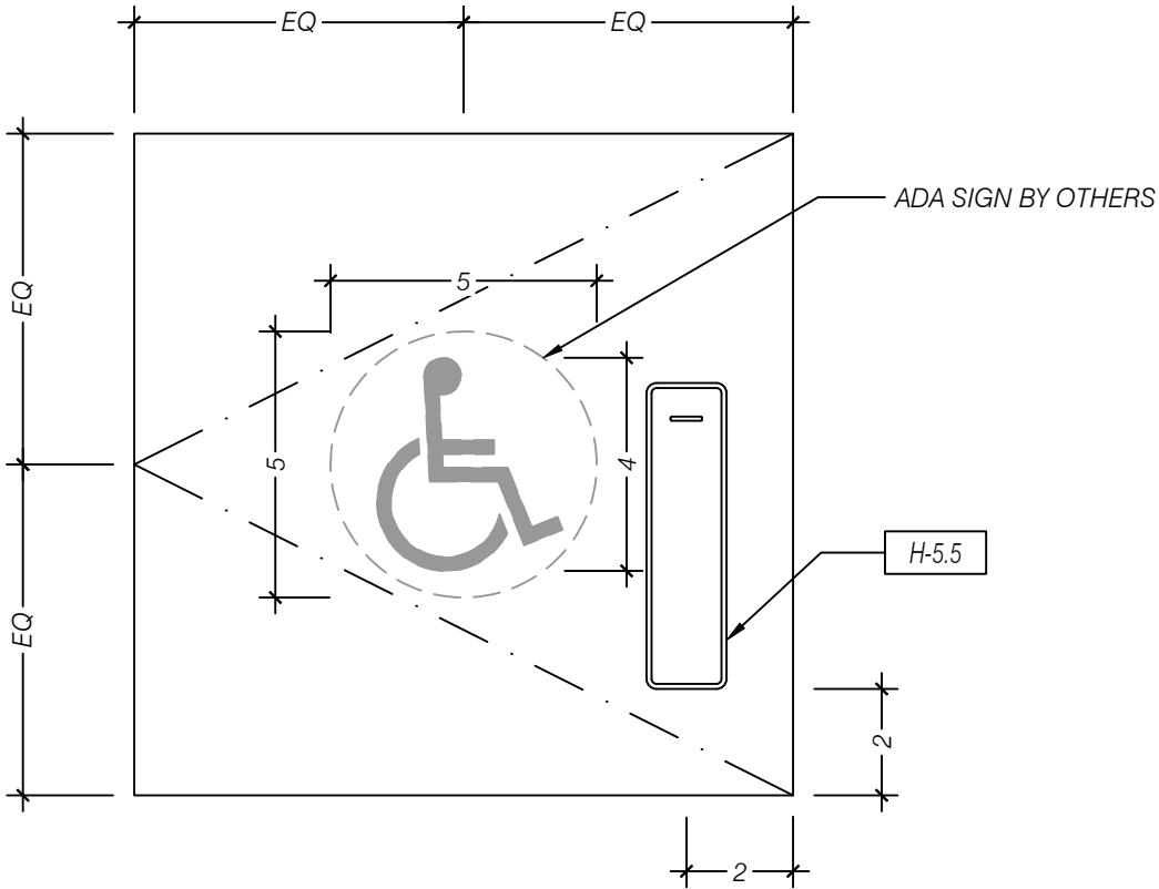
A ENLARGED DETAIL - LOCK LOCATION SCALE 1:4 (3"=1'-0") ARCH REF: NA
