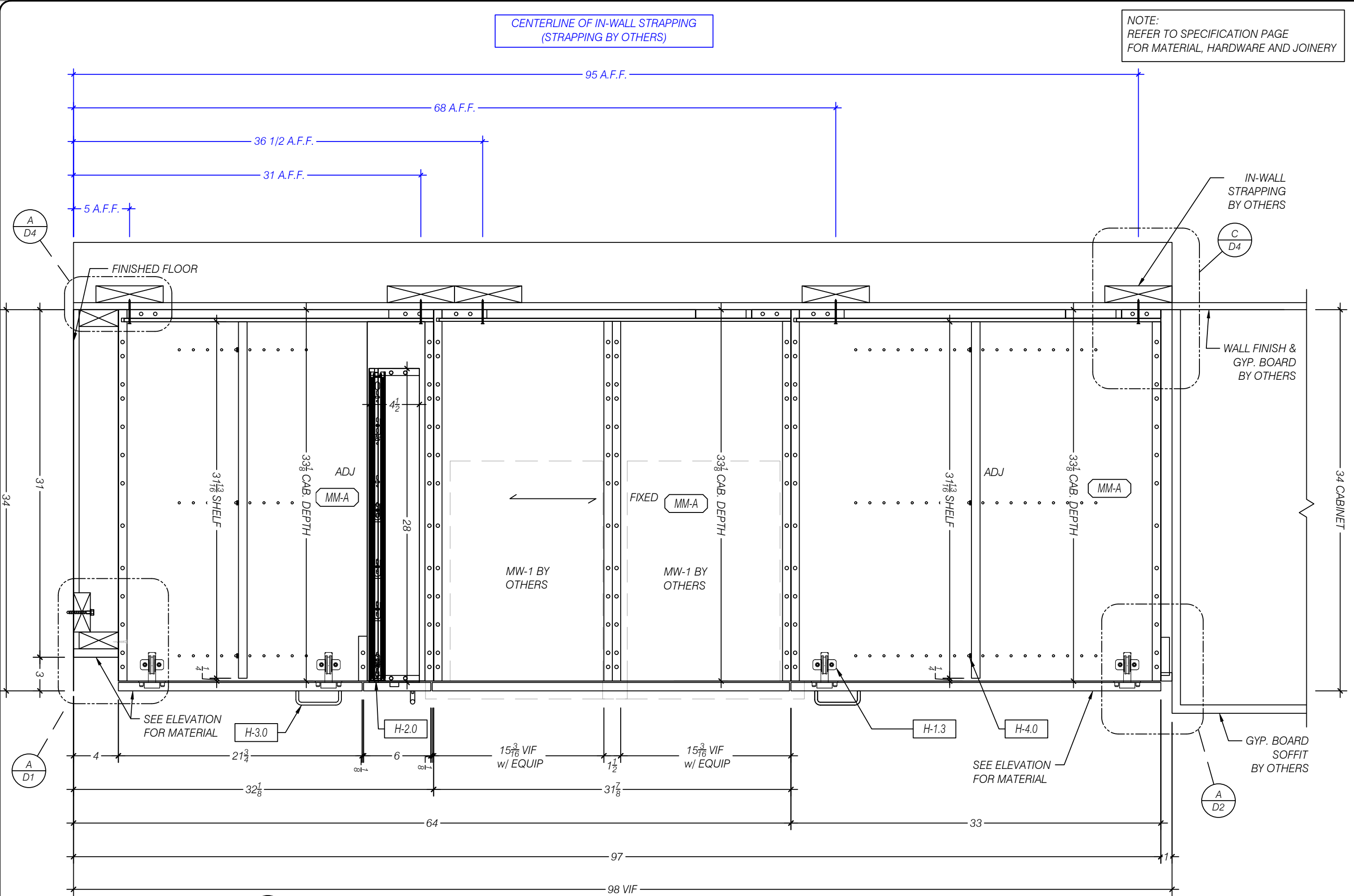
A SECTION - TALL CABINET SCALE 1:8 (1 1/2"=1'-0") ARCH REF: 22/AE582
