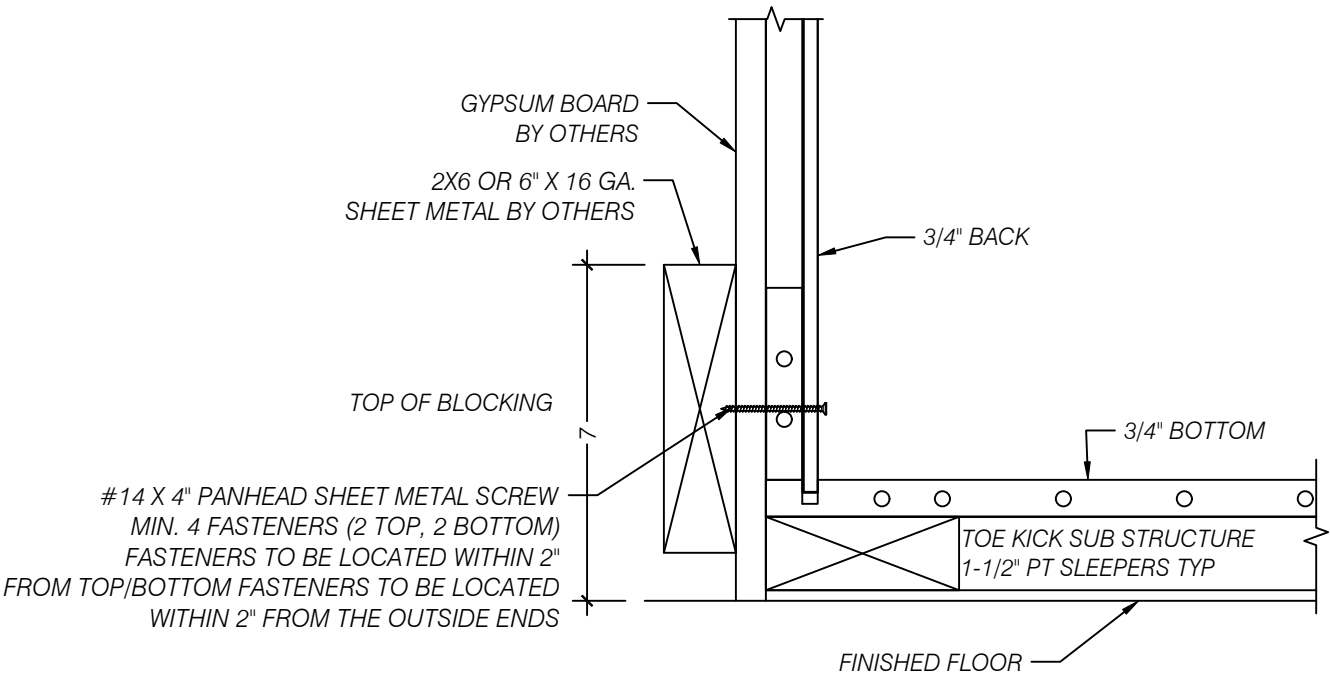
C ENLARGED DETAIL - THICK BACK CABINET ATTACHEMENT @ WALL SCALE 1:4 (3"=1'-0") ARCH REF: NA
