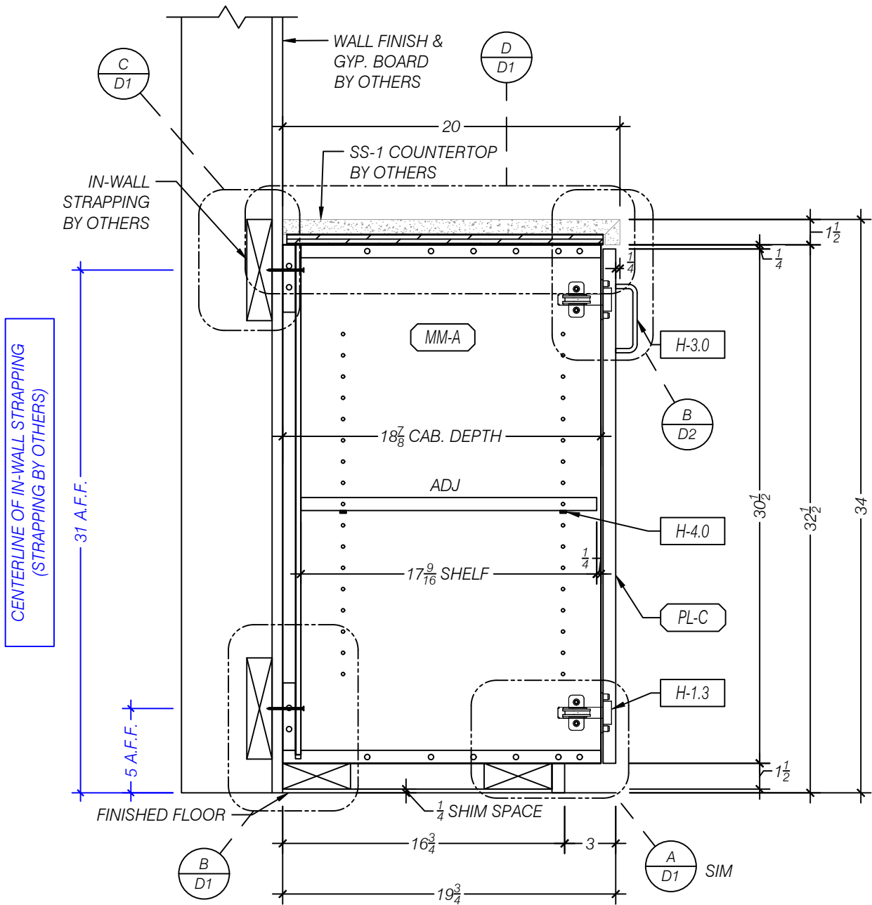
A SECTION - BASE CABINET SCALE 1:8 (1 1/2"=1'-0") ARCH REF: 15/AE581 (SIM)
