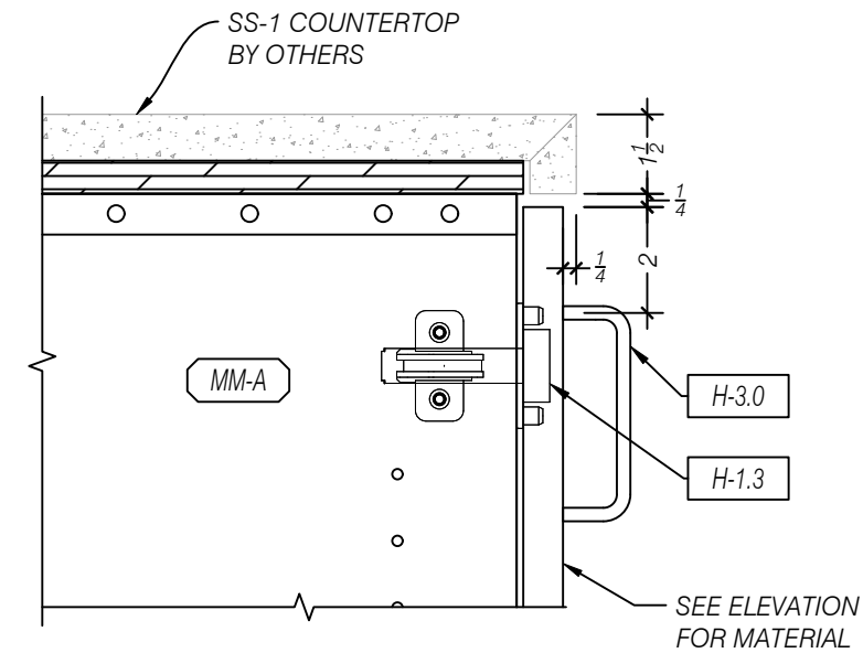
B ENLARGED DETAIL - DOOR PULL LOCATION SCALE 1:4 (3"=1'-0") ARCH REF: NA
