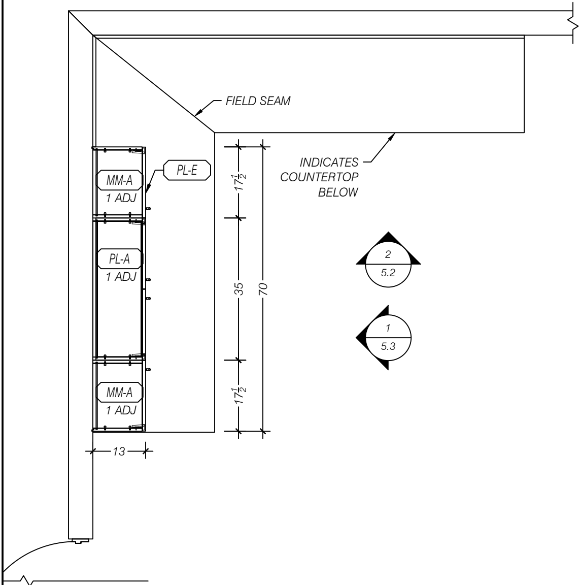
1 PLAN SECTION WALL - MEDIA CONTROL 113 SCALE 1:24 (1/2"=1'-0") ARCH REF: NA
