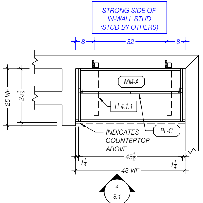
3 PLAN SECTION - ALL GENDER 103 SCALE 1:24 (1/2"=1'-0") ARCH REF: NA
