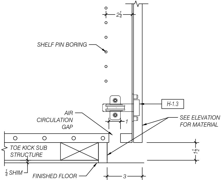
A ENLARGED DETAIL - TOE KICK FACE SCALE 1:4 (3"=1'-0") ARCH REF: 11/AE584
