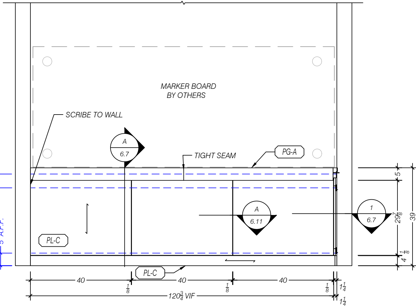
2 ELEVATION NORTH - BREAK ROOM 115 SCALE 1:24 (1/2"=1'-0") ARCH REF: 2/AE407
