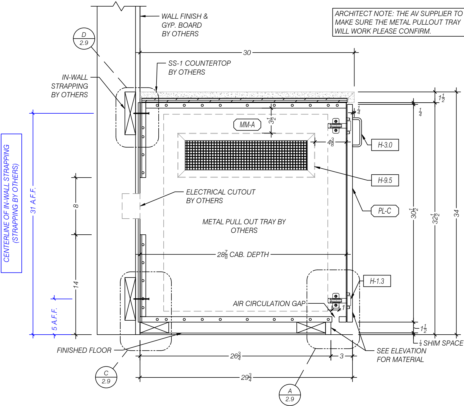
A SECTION - BASE CABINET SCALE 1:8 (1 1/2"=1'-0") ARCH REF: 10/AE581
