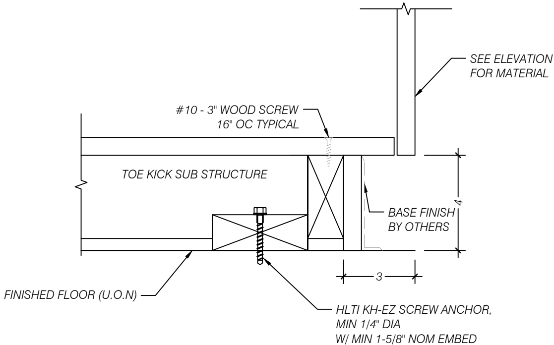
A ENLARGED DETAIL - TYPICAL TOE KICK FACE SCALE 1:4 (3"=1'-0") ARCH REF: 11/AE584
