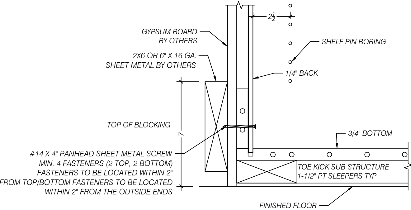
B ENLARGED DETAIL - BASE CABINET ATTACHEMENT @ WALL SCALE 1:4 (3"=1'-0") ARCH REF: NA
