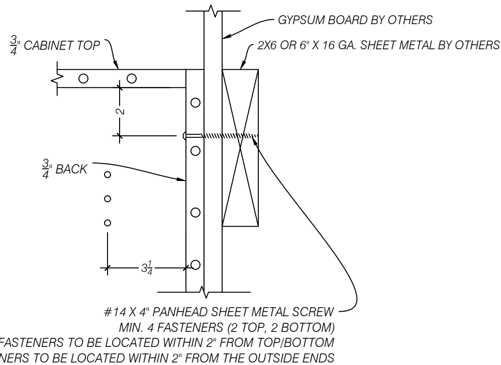
C ENLARGED DETAIL - THICK BACK CABINET ATTACHEMENT @ WALL SCALE 1:4 (3"=1'-0") ARCH REF: NA
