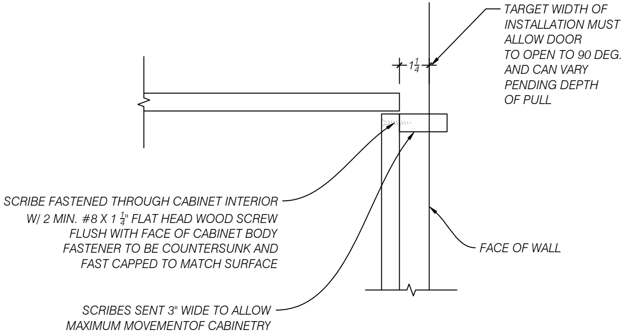
B ENLARGED DETAIL - CASEWORK SCRIBE @ WALL SCALE 1:4 (3"=1'-0") ARCH REF: NA
