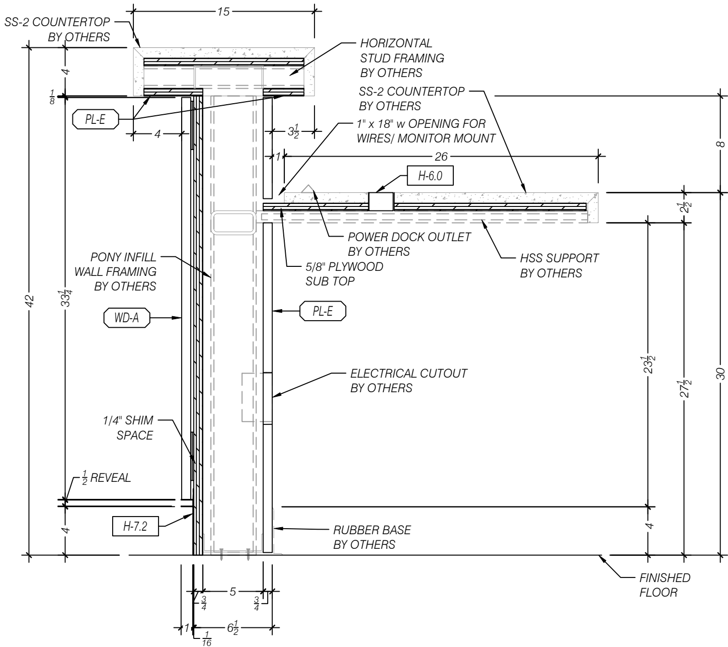
A SECTION - COUNTERTOP w/ TRANSACTION COUNTER SCALE 1:8 (1 1/2"=1'-0") ARCH REF: 3/AE584
