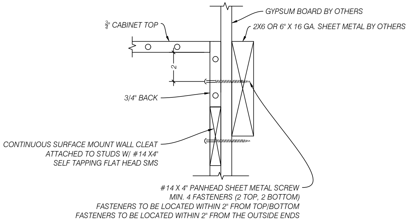
A ENLARGED DETAIL - THICK BACK WALL CABINET ATTACHMENT @ WALL SCALE 1:4 (3"=1'-0") ARCH REF: NA
