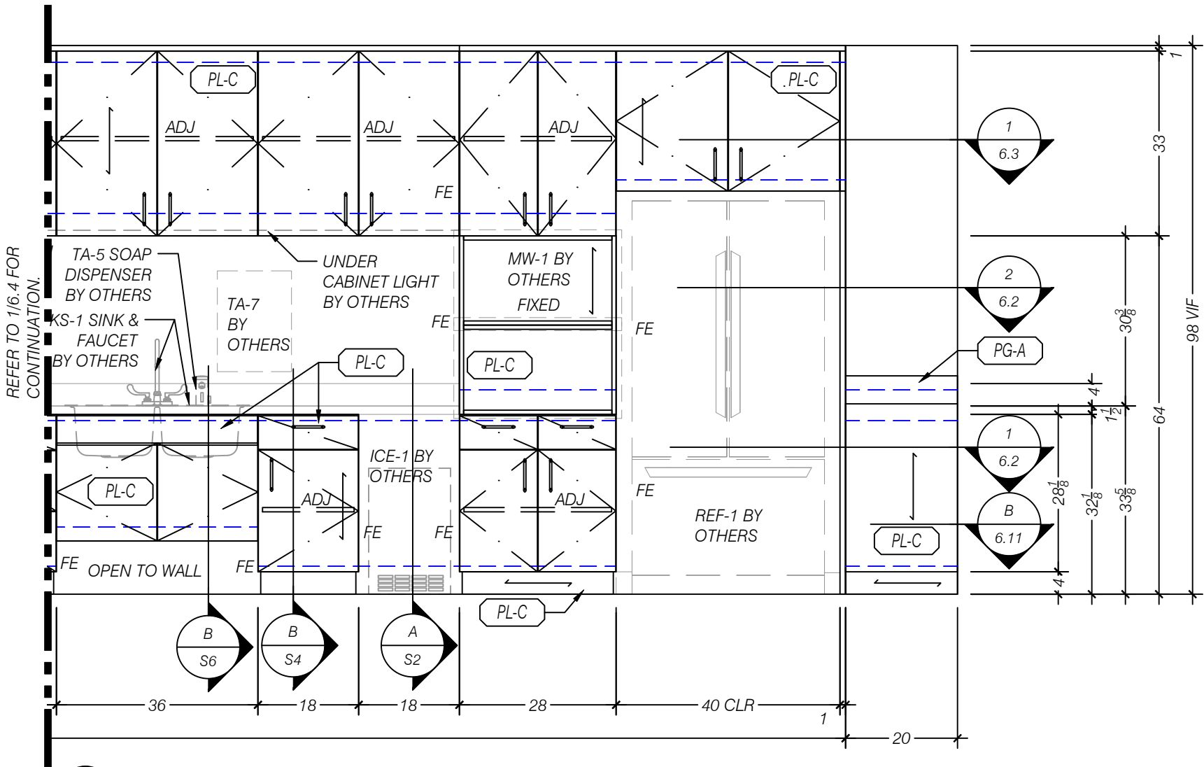
1 ELEVATION EAST - BREAK ROOM 115 SCALE 1:24 (1/2"=1'-0") ARCH REF: 3/AE407
