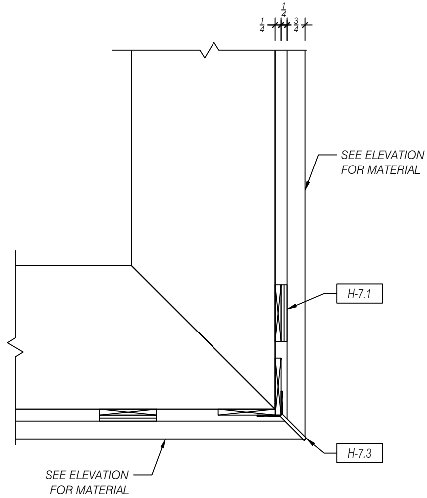
C ENLARGED DETAIL - P-LAM VERTICAL CORNER TRIM SCALE 1:4 (3"=1'-0") ARCH REF: 9/584
