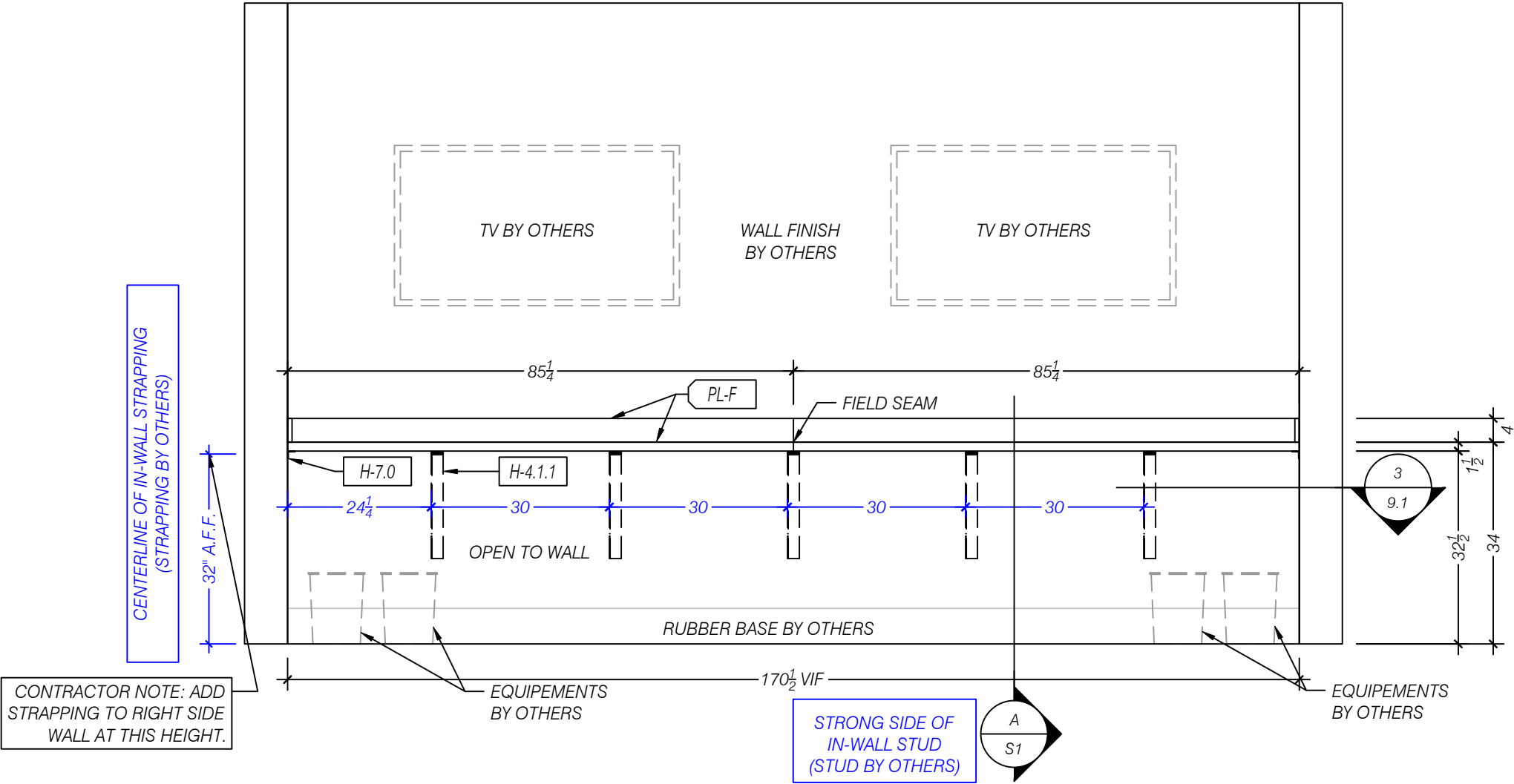
1 ELEVATION WEST - AV COORDINATION ROOM 126 SCALE 1:24 (1/2"=1'-0") ARCH REF: 16/AE408
