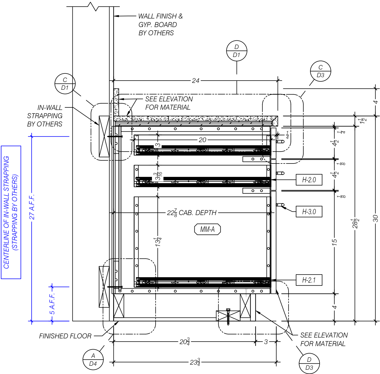
A SECTION - 3 DRAWER CABINET SCALE 1:8 (1 1/2"=1'-0") ARCH REF: 2/AE583
