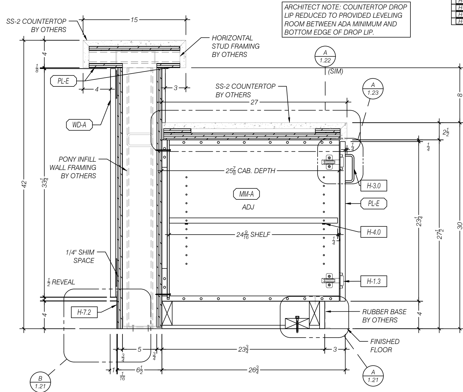
A SECTION - BASE CABINET w/ TRANSACTION COUNTER SCALE 1:8 (1 1/2"=1'-0") ARCH REF: 4/AE584
